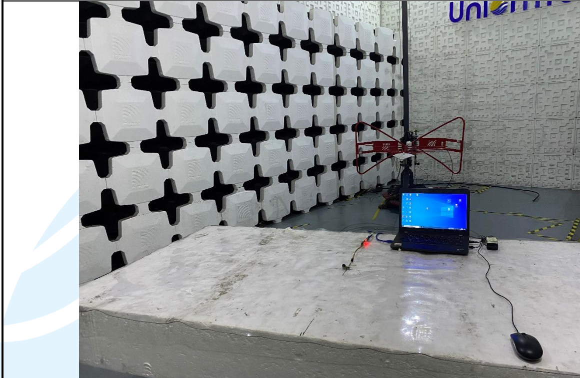
Radiated emission Test Setup (30 MHz~1 GHz) _Left earbuds
