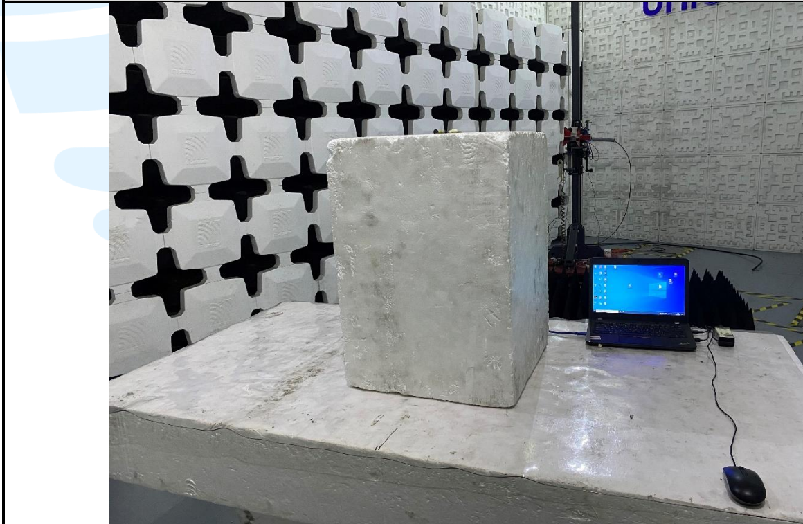
Radiated emission Test Setup (Above 1 GHz) _Left earbuds
