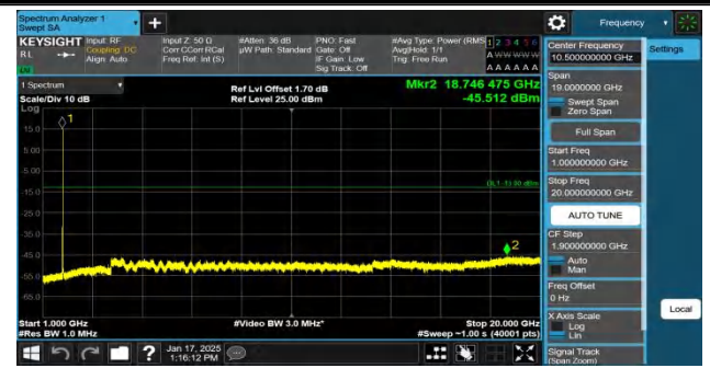
Band4-1513-4-1000~20000MHz-PASS
