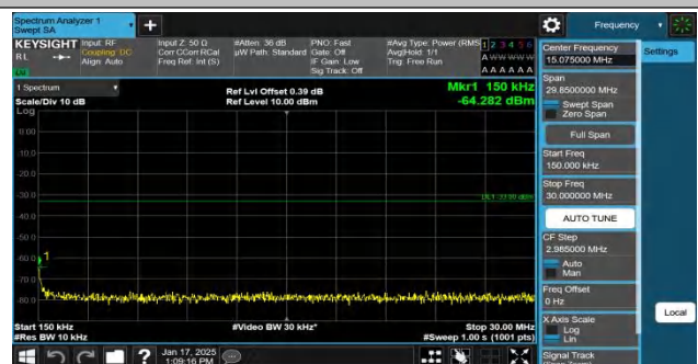
Band4-1312-2-0.15~30MHz-PASS
