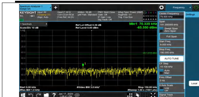
Band4-1312-1-0.009~0.15MHz-PASS
