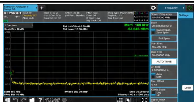
Band4-1312-1-0.15~30MHz-PASS
