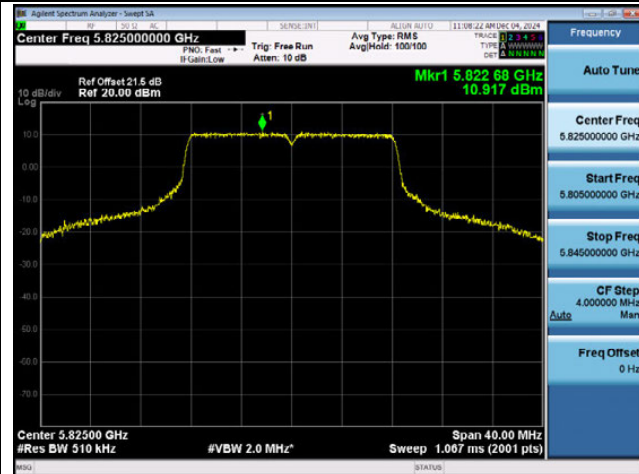
802.11ac-VHT20 Power Spectral Density - Ant 1
