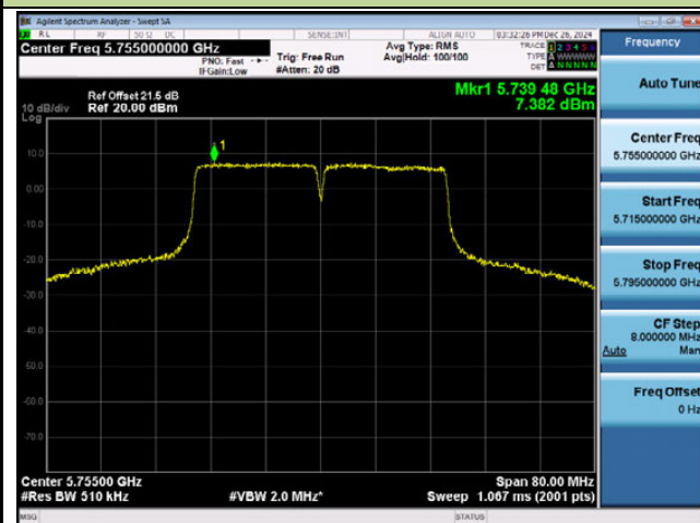
802.11ac-VHT80 Power Spectral Density - Ant 1
