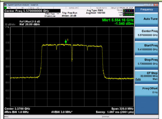
Channel 114 (5570MHz)
