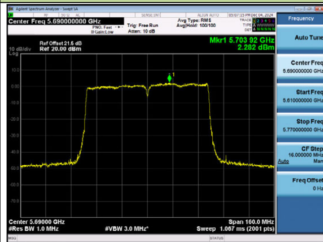
802.11ac-VHT160 Power Spectral Density - Ant 1
