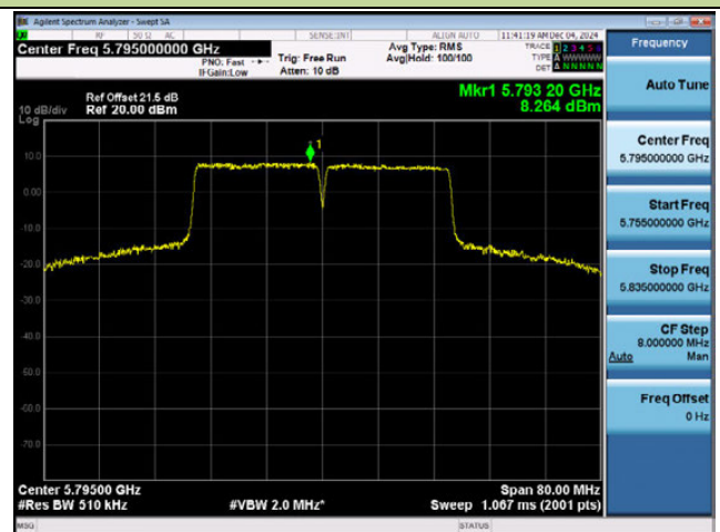
802.11ac-VHT80 Power Spectral Density - Ant 1
