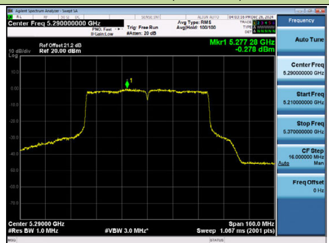
Channel 58 (5290MHz)
