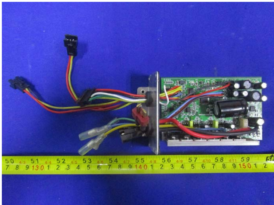
EUT – Motor Mainboard Top View
