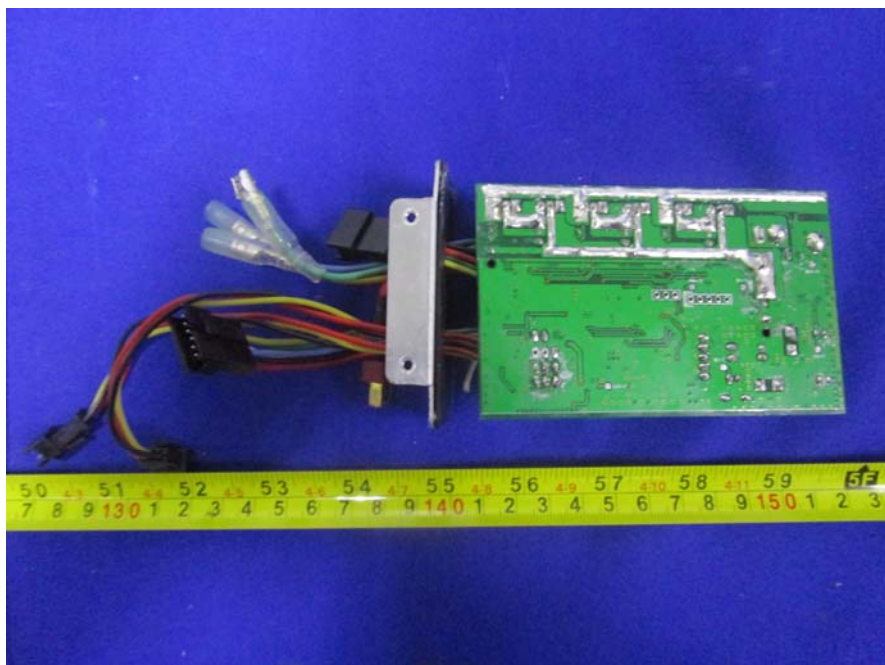
EUT – Motor Mainboard Bottom View
