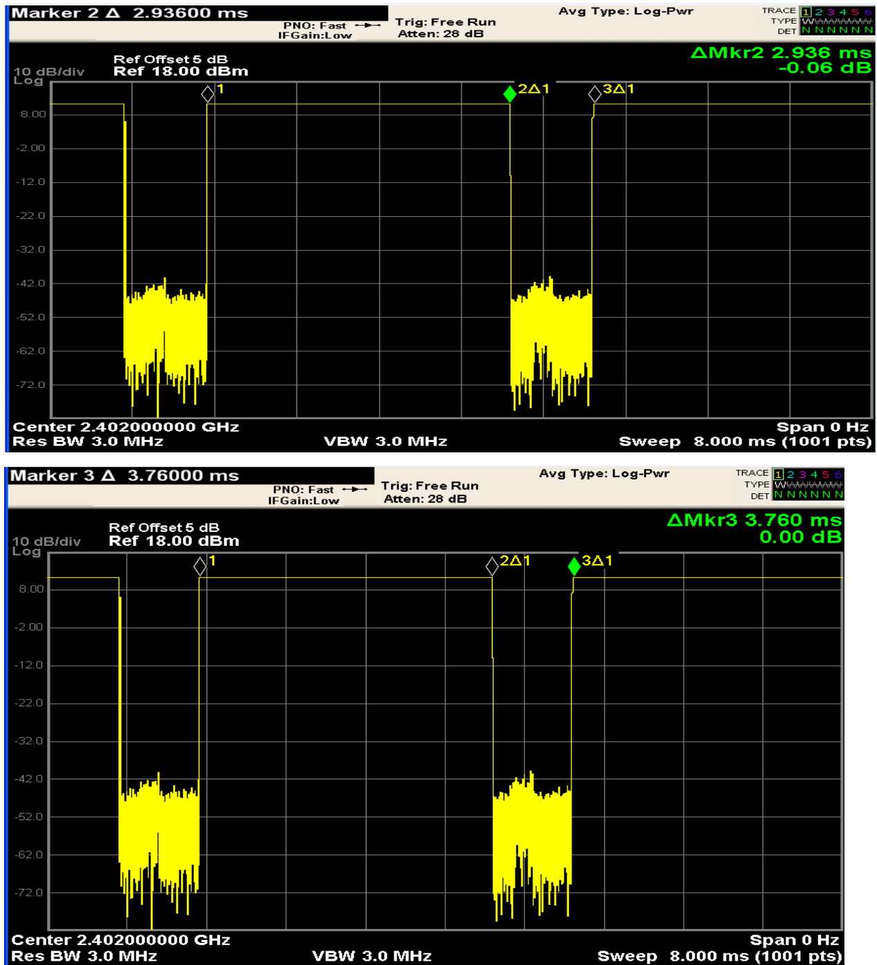
Figure: Bluetooth Transmission Plot
