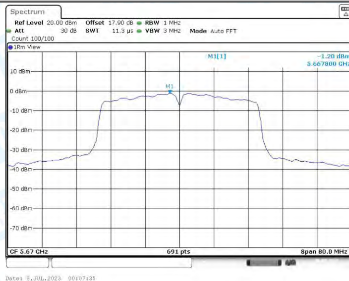
11N40-CDD_Ant4_5670
