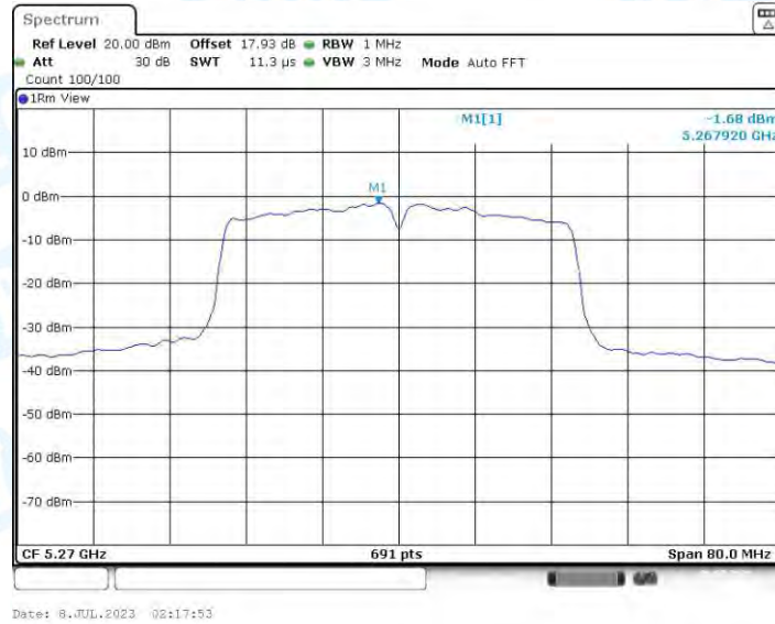
11AC40-CDD_Ant4_5270
