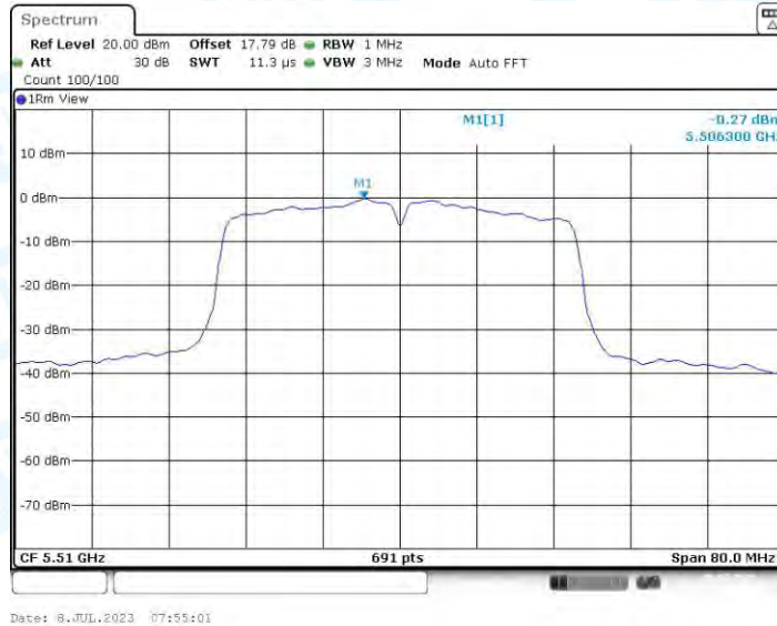
11AC40-CDD_Ant3_5510
