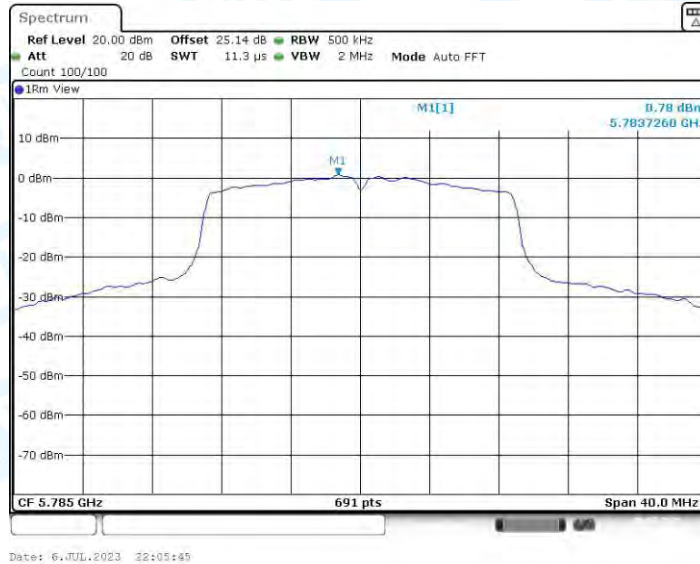
11AC20-CDD_Ant2_5785
