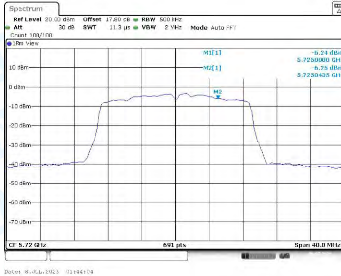
11AC20-CDD_Ant4_5720_UNII-3
