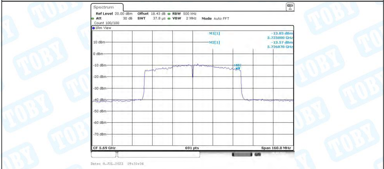
11AC80-CDD_Ant4_5690_UNII-3
