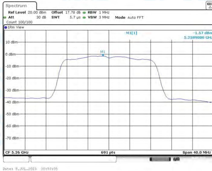
11AC20-CDD_Ant4_5260
