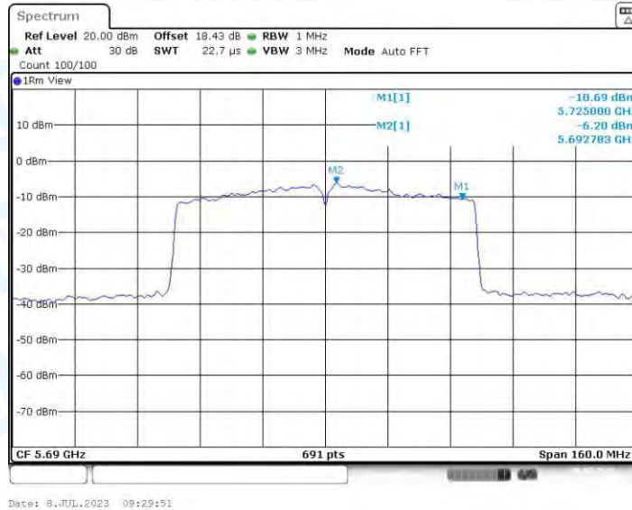
11AC80-CDD_Ant1_5690_UNII-3
