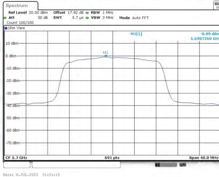
11AC20-CDD_Ant4_5700
