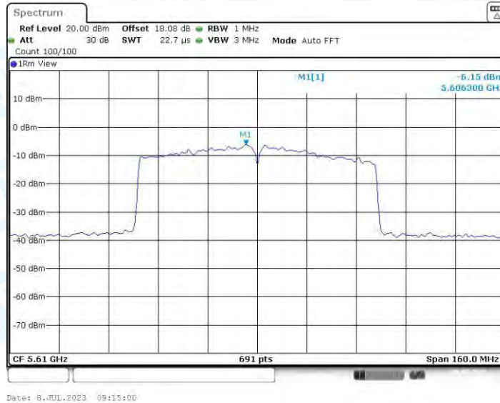
11AC80-CDD_Ant4_5610
