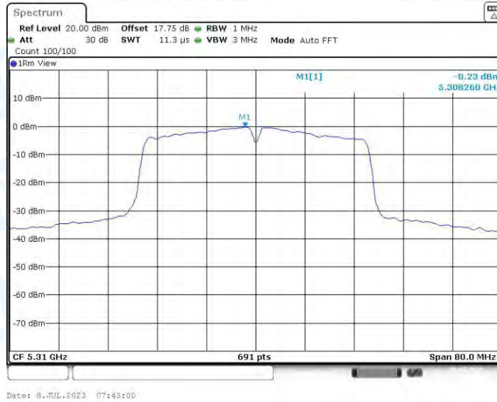
11AC40-CDD_Ant3_5310
