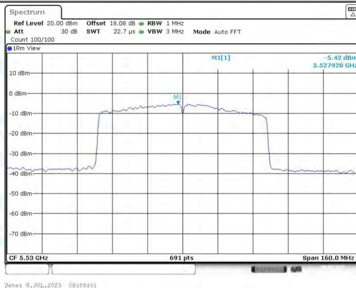
11AC80-CDD_Ant3_5530
