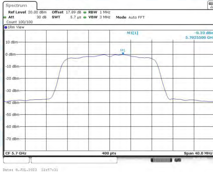
11N20-BF_Ant4_5700
