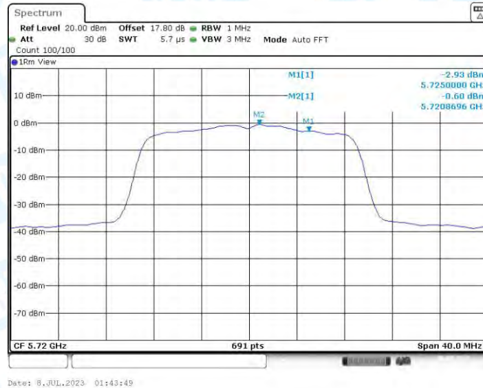
11AC20-CDD_Ant4_5720_UNII-2C
