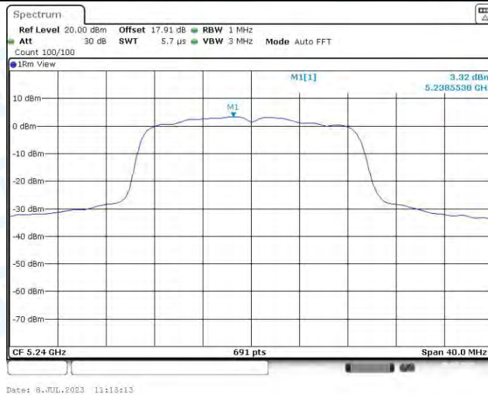
11N20-BF_Ant4_5240
