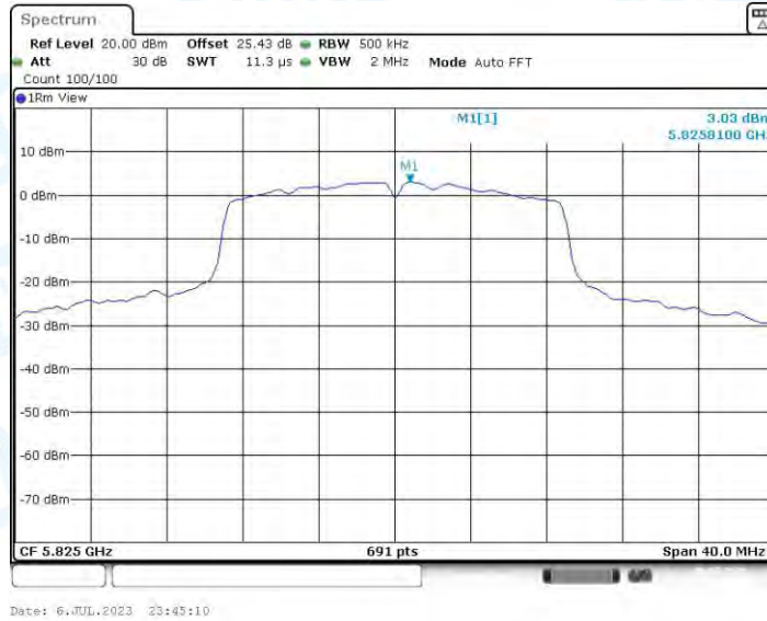
11N20-BF_Ant4_5825
