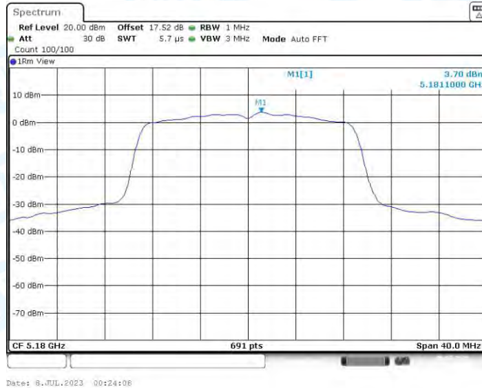
11AC20-CDD_Ant3_5180
