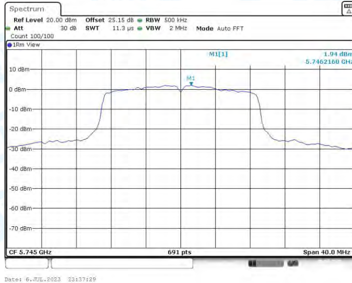
11N20-BF_Ant4_5745
