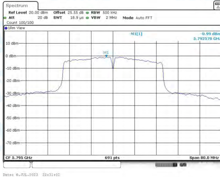
11AC40-CDD_Ant4_5795
