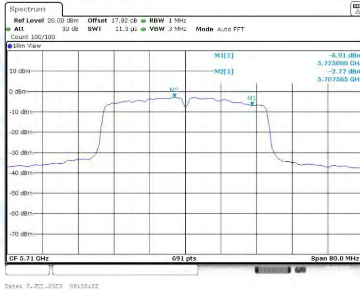
11AC40-CDD_Ant2_5710_UNII-2C
