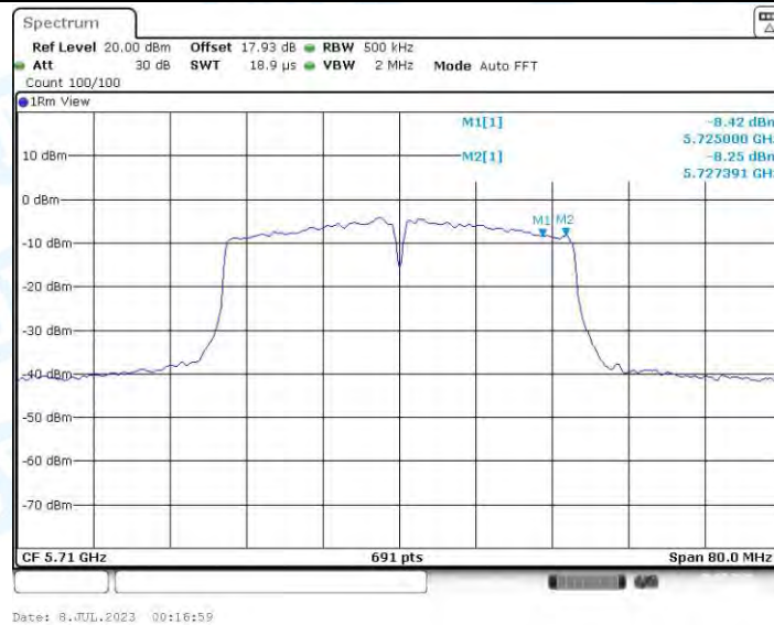
11N40-CDD_Ant4_5710_UNII-3
