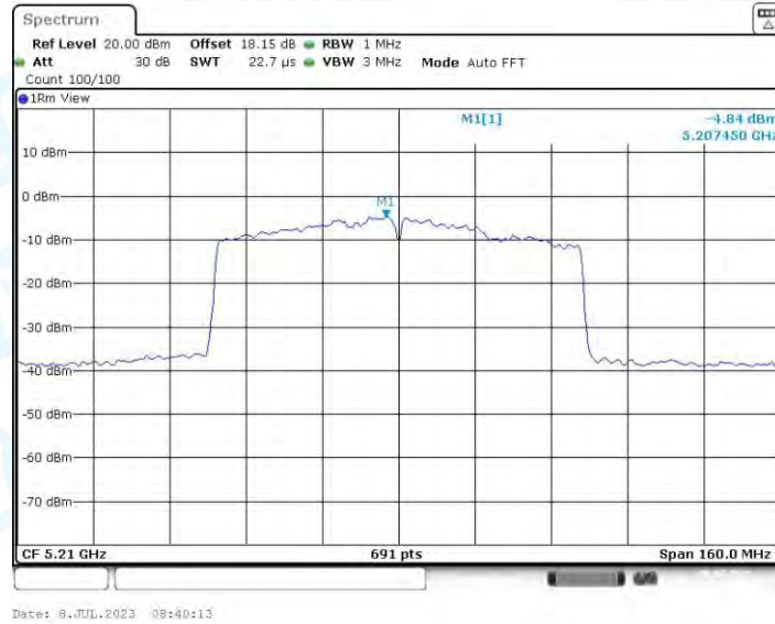
11AC80-CDD_Ant3_5210
