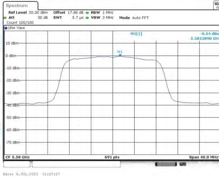
11AC20-CDD_Ant4_5580
