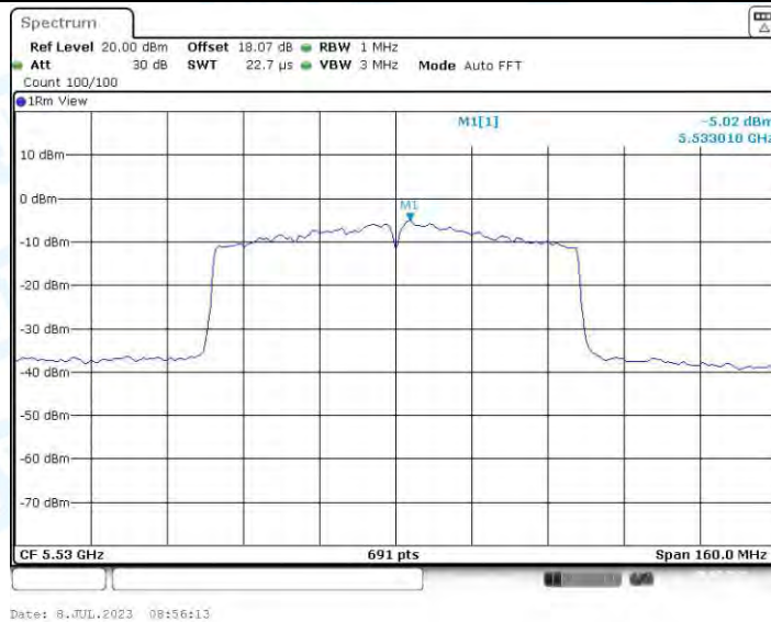
11AC80-CDD_Ant2_5530
