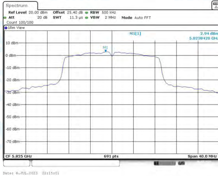
11AC20-CDD_Ant3_5825
