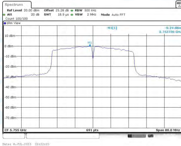
11AC40-CDD_Ant3_5755
