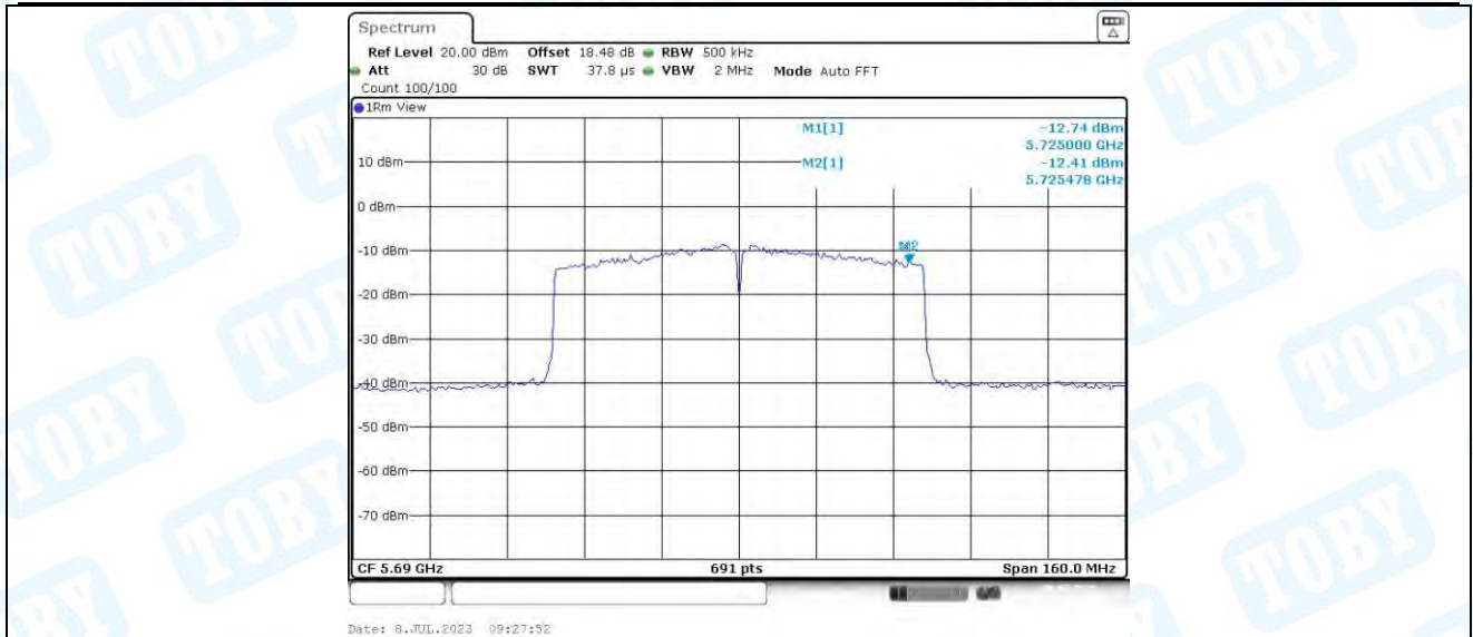
11AC80-CDD_Ant4_5690_UNII-3
