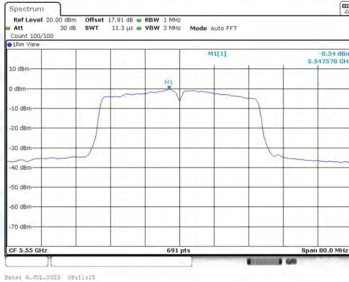
11AC40-CDD_Ant2_5550
