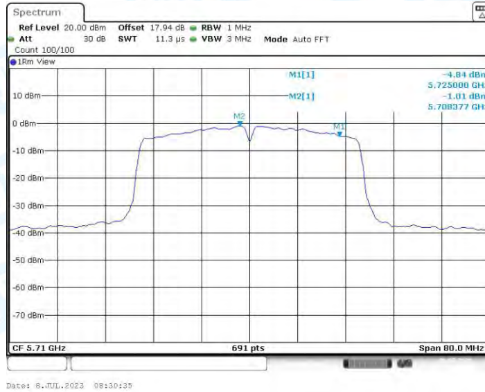
11AC40-CDD_Ant3_5710_UNII-2C
