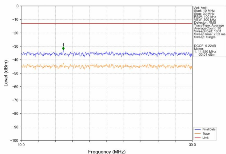
PCS1900 EGPRS LCH 1850.2MHz 1 TX Slot NTN
