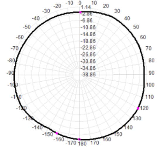
Total(H-XY), Max= 1.14dBi, CirD=3.58
