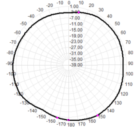
Total(H-XY), Max= 0.63dBi, CirD=4.38
