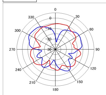
2570MHz (B7) Red:Vertical
