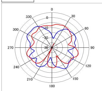
2690MHz Red:Vertical
