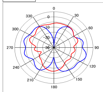
1850MHz Red:Vertical
