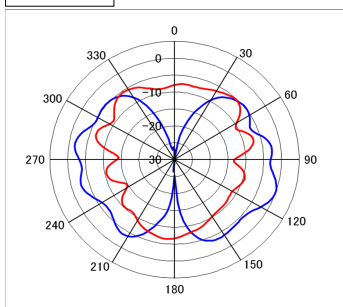
1915MHz Red:Vertical
