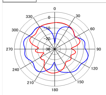
1780MHz Red:Vertical
