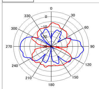
3550MHz Red:Vertical
