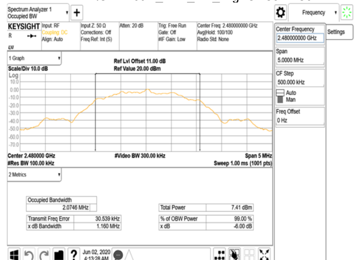
BLE 2M OBW 6dB_BLE_2M_HighCH39-2480
