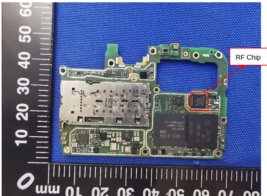
MAIN BOARD REAR VIEW (WITHOUT SHIELDING)
