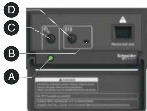
PD100 with cover open
