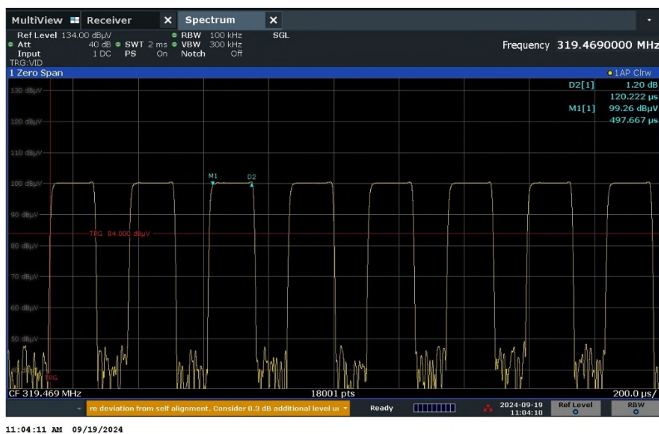
Figure 2-4 – Pulse Width 1
