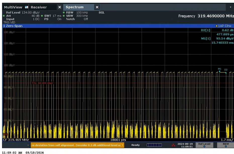
Figure 2-5 – Pulse Width 2
