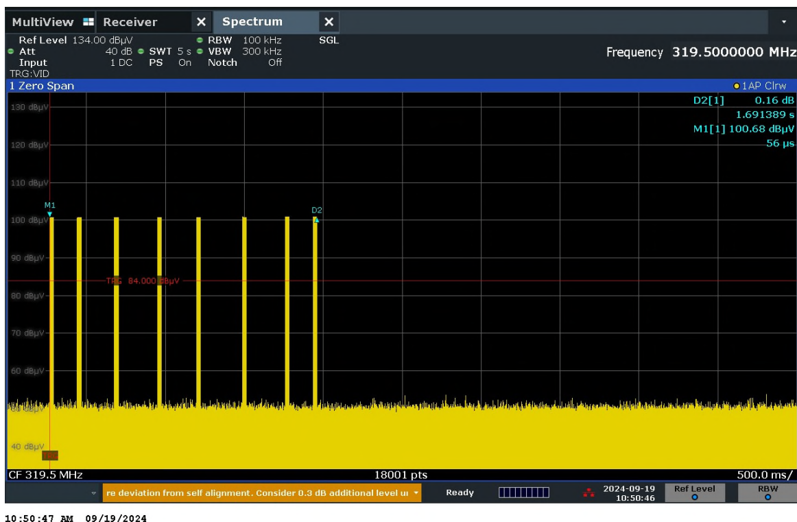
Figure 2-1 – Deactivation Period
