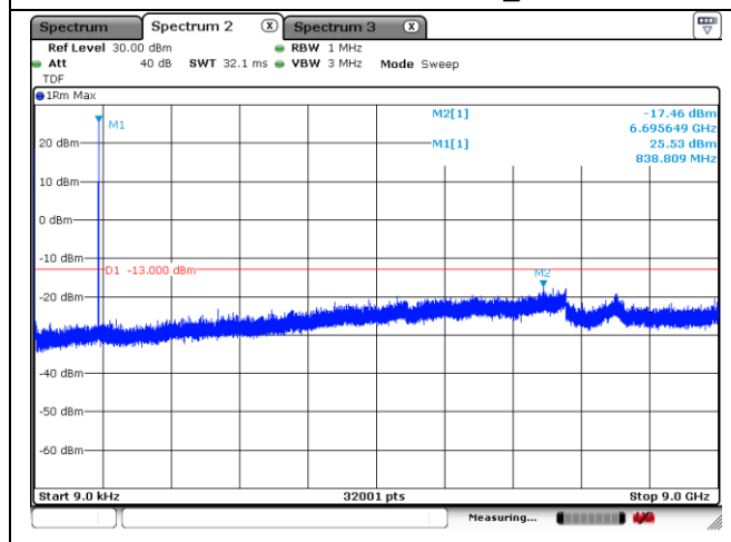
PCC 10 MHz RB1 + SCC 5 MHz RB1_Middle Channel
