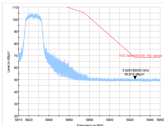
802.11a-Channel 165: Peak
