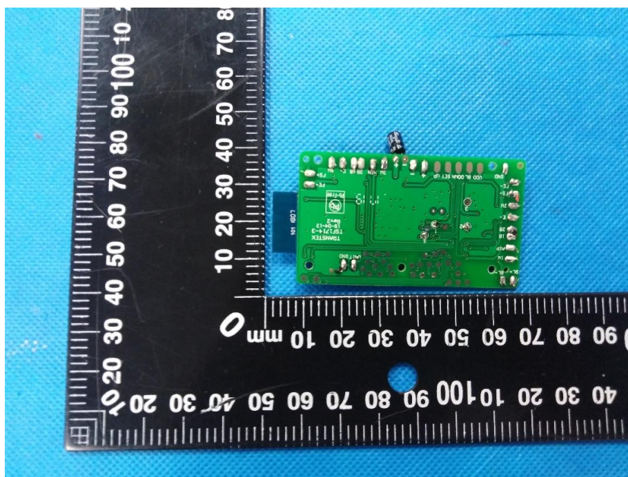
WiFi Antenna
