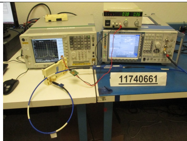
FREQUENCY STABILITY
