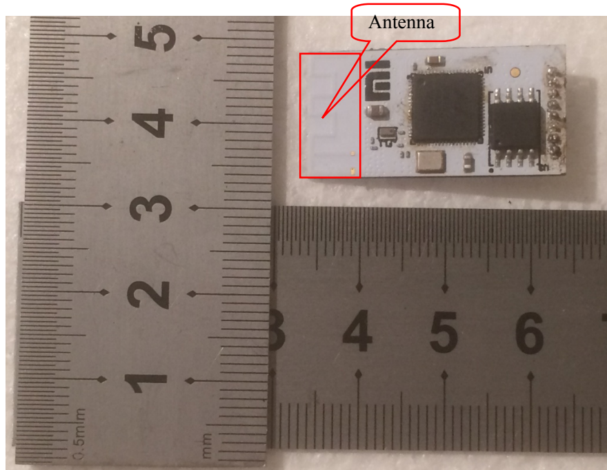
EUT – WIFI Module Top View
