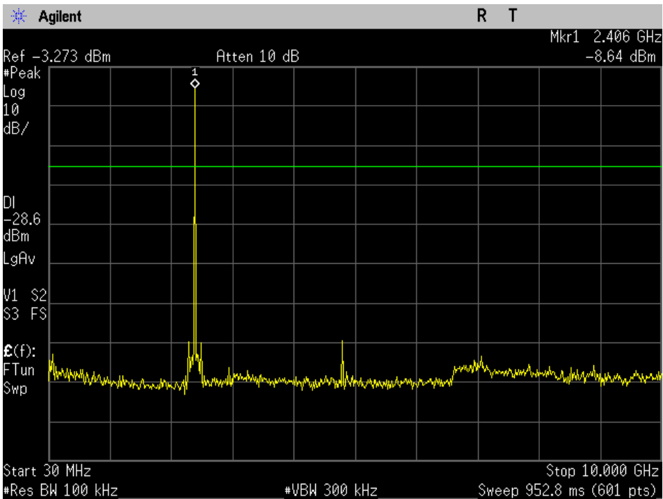
Low Channel (2402 MHz), 30 MHz to 10000 MHz
