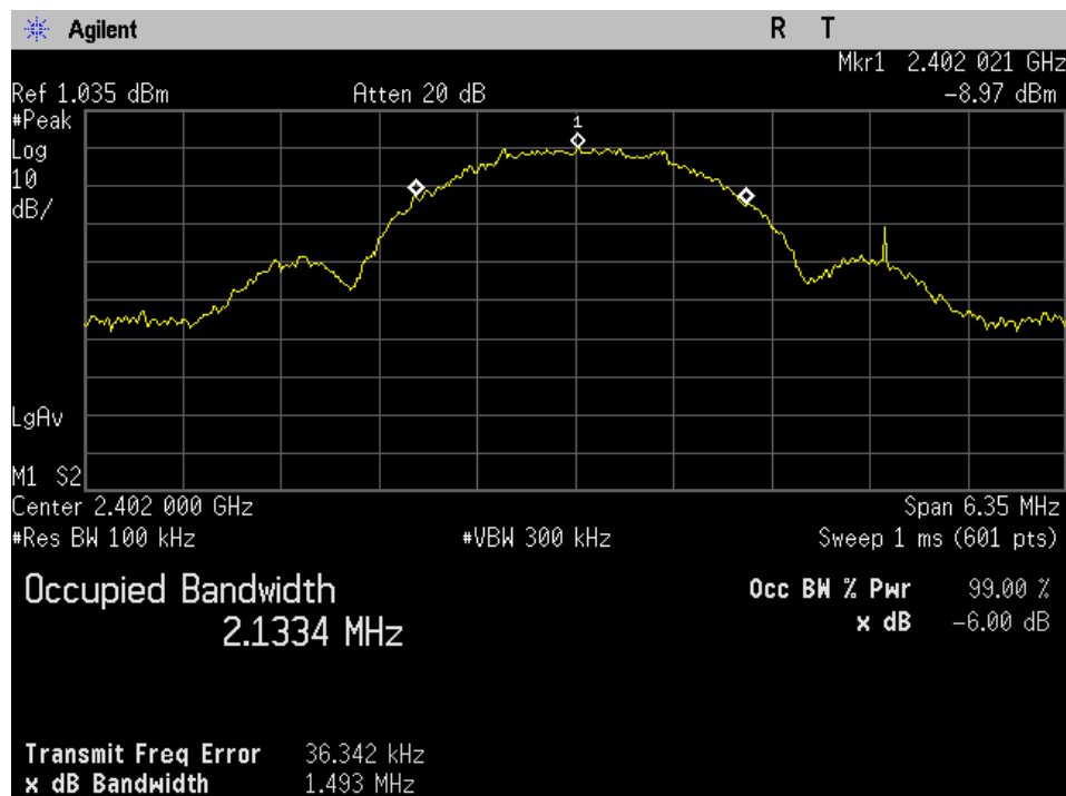
Low Channel (2402 MHz), -6 dB OBW
