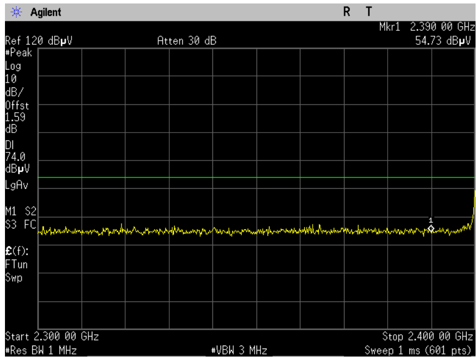
Low Channel (2402 MHz) Peak
