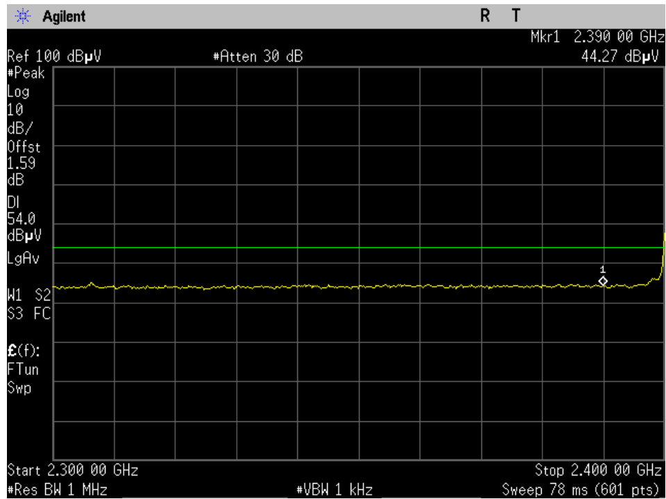
Low Channel (2402 MHz) Average
