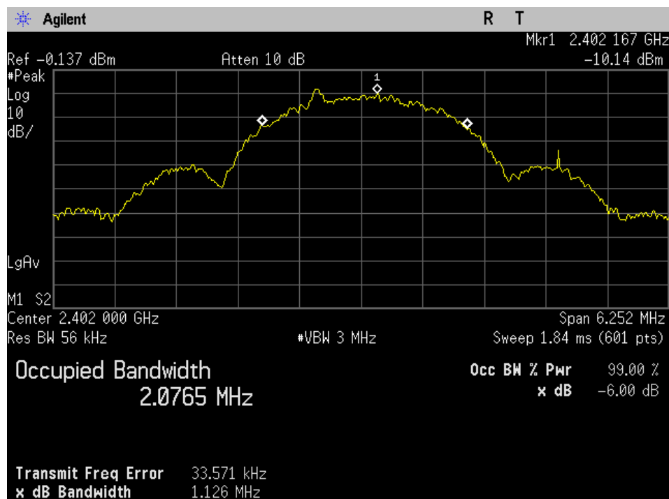
Low Channel (2402 MHz), 99% OBW
