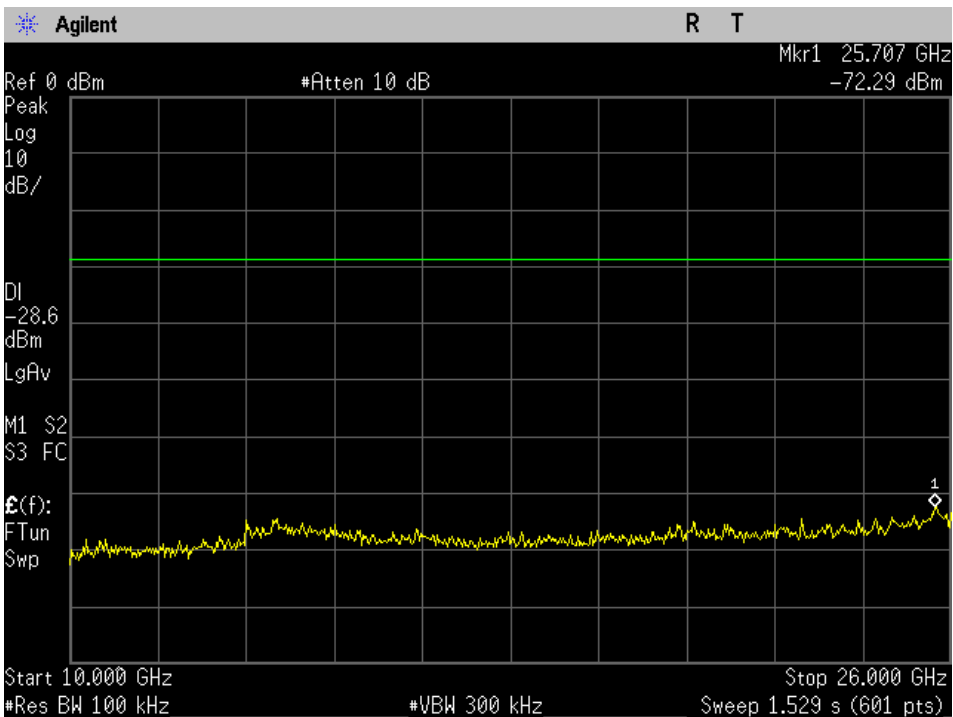
Low Channel (2402 MHz), 10000 MHz to 26000 MHz
