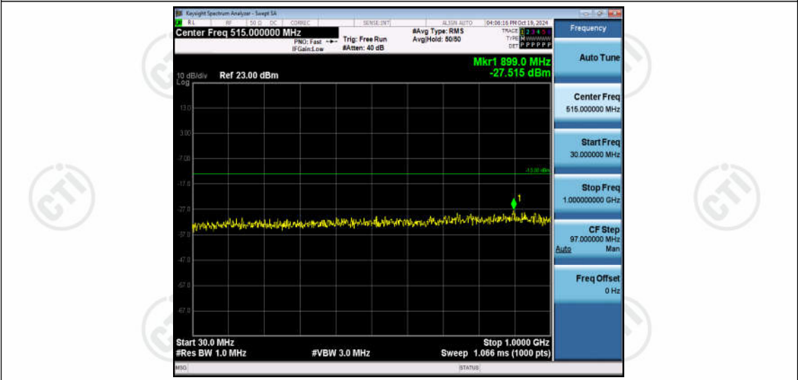
Band2-5MHz-16QAM-19175-1RB#0-Range1:30~1000MHz
