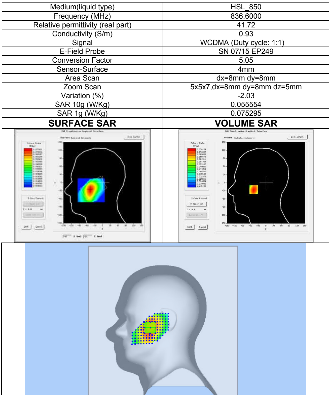
Plot 7: WCDMA BAND V, Middle channel (Right Head Cheek) Product Description: MOBILE PHONE Test Date: Mar 27,2017
