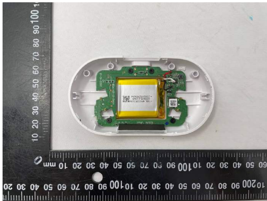
Figure 7: Internal view-2 (charging case)
