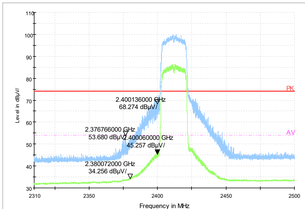
Fig.33 Frequency Band Edge: Ch1,11n(20M)
