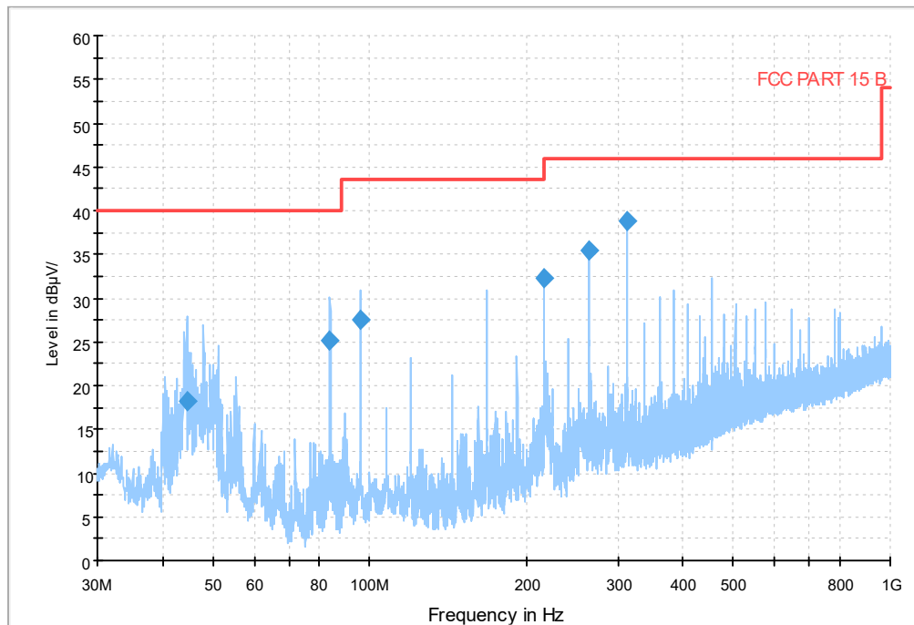
Fig.67 Radiated emission: Ch11, 30MHz-1GHz
