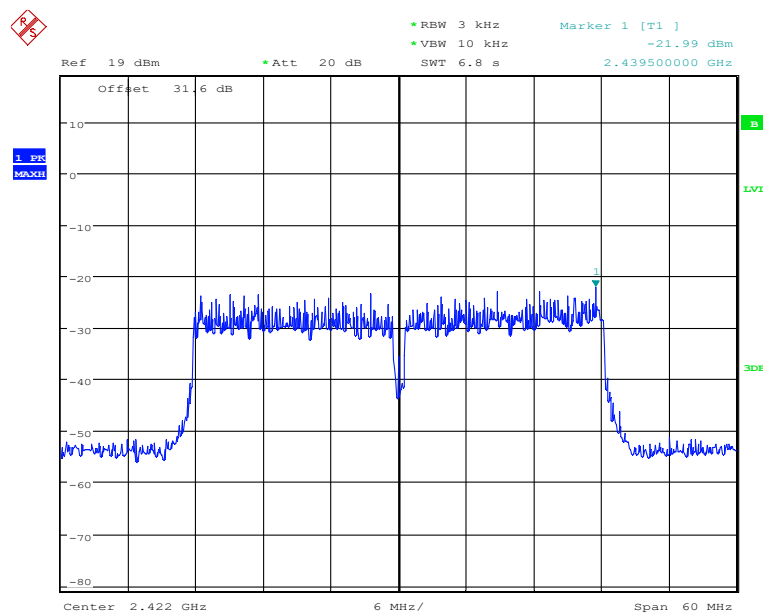
Fig.7 Power spectral density: CH1,1n
