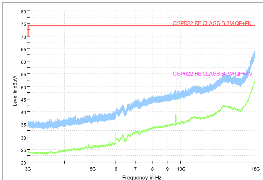
Fig.69 Radiated emission: Ch11, 3GHz-18GHz
