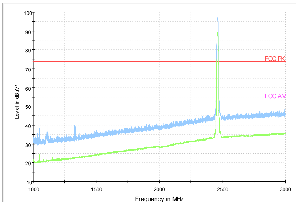
Fig.68 Radiated emission: Ch11, 1GHz-3GHz
