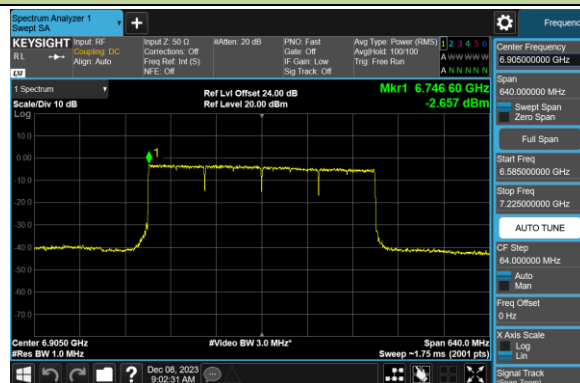
Channel 191 (6905MHz)
