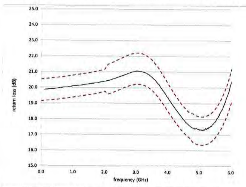
Fig. 3: Result of 20 dB mismatch with single uncertainty limit of its calibration.
