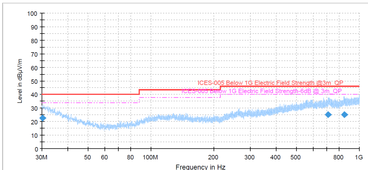
Figure 5: Spectral Diagrams, Radiated Emission, 30MHz-1000MHz, Horizontal polarization by adapter
