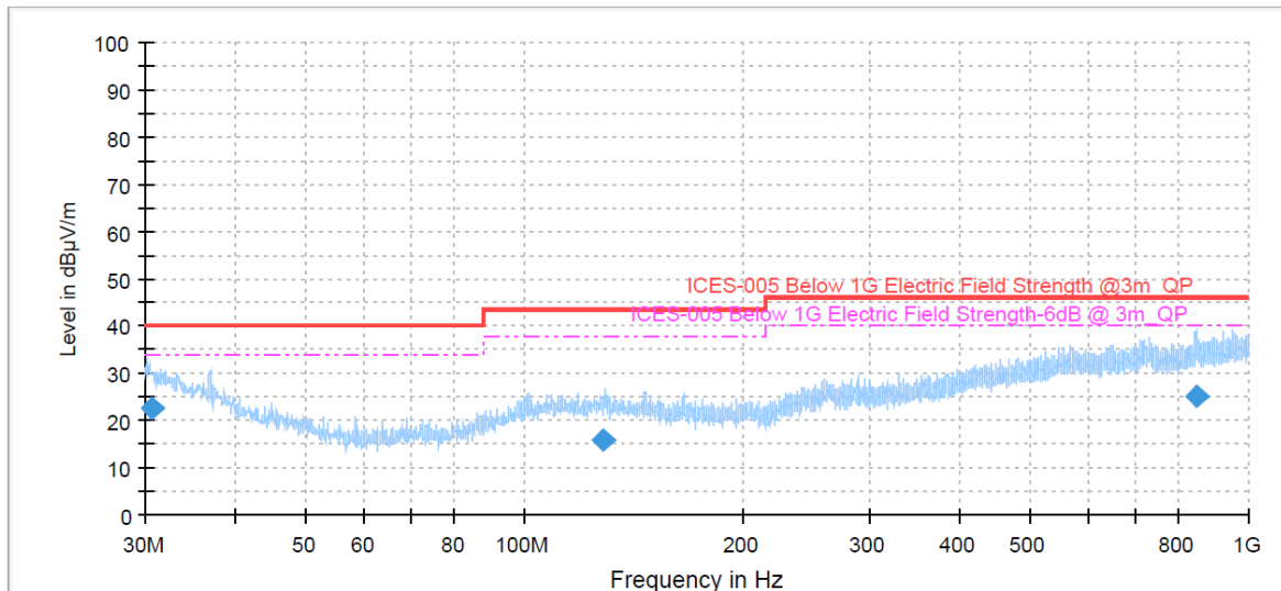
Figure 8: Spectral Diagrams, Radiated Emission, 30MHz-1000MHz, Vertical polarization by battery
