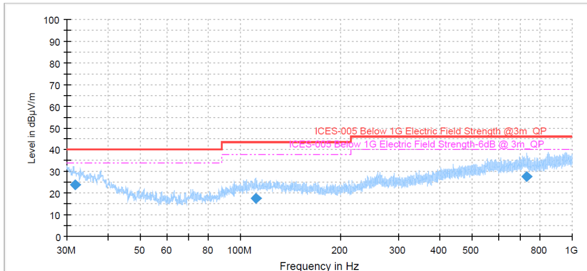
Figure 6: Spectral Diagrams, Radiated Emission, 30MHz-1000MHz, Vertical polarization by adapter
