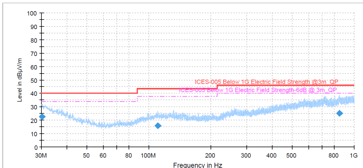
Figure 7: Spectral Diagrams, Radiated Emission, 30MHz-1000MHz, Horizontal polarization by battery
