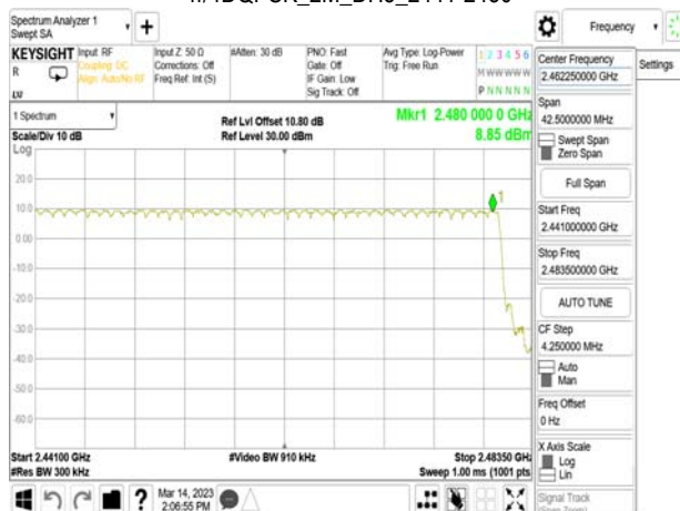
\pi/4 DQPSK_2M_DH5_2441-2480
