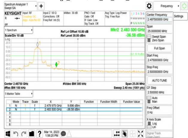
Band Edge_π/4DQPSK_2M_DH5_2480MHz
