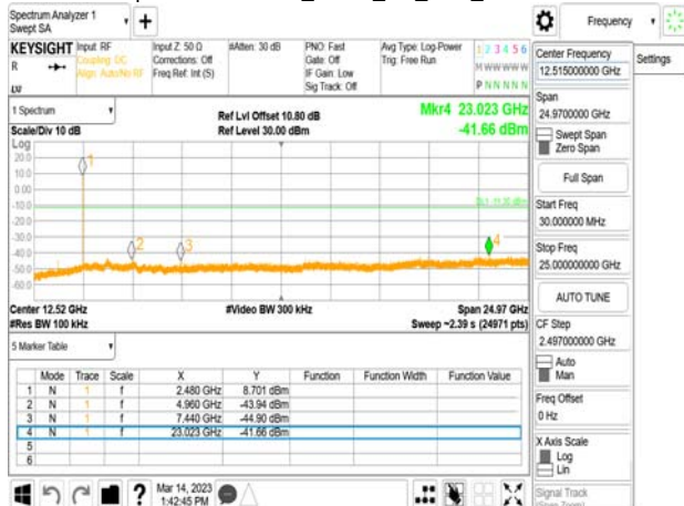
Spurious Emission_GFSK_1M_DH5_2480MHz
