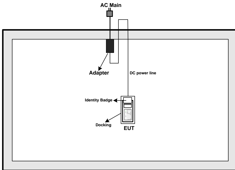
Test Setup Diagram - Radiated Test (Above 30MHz)
