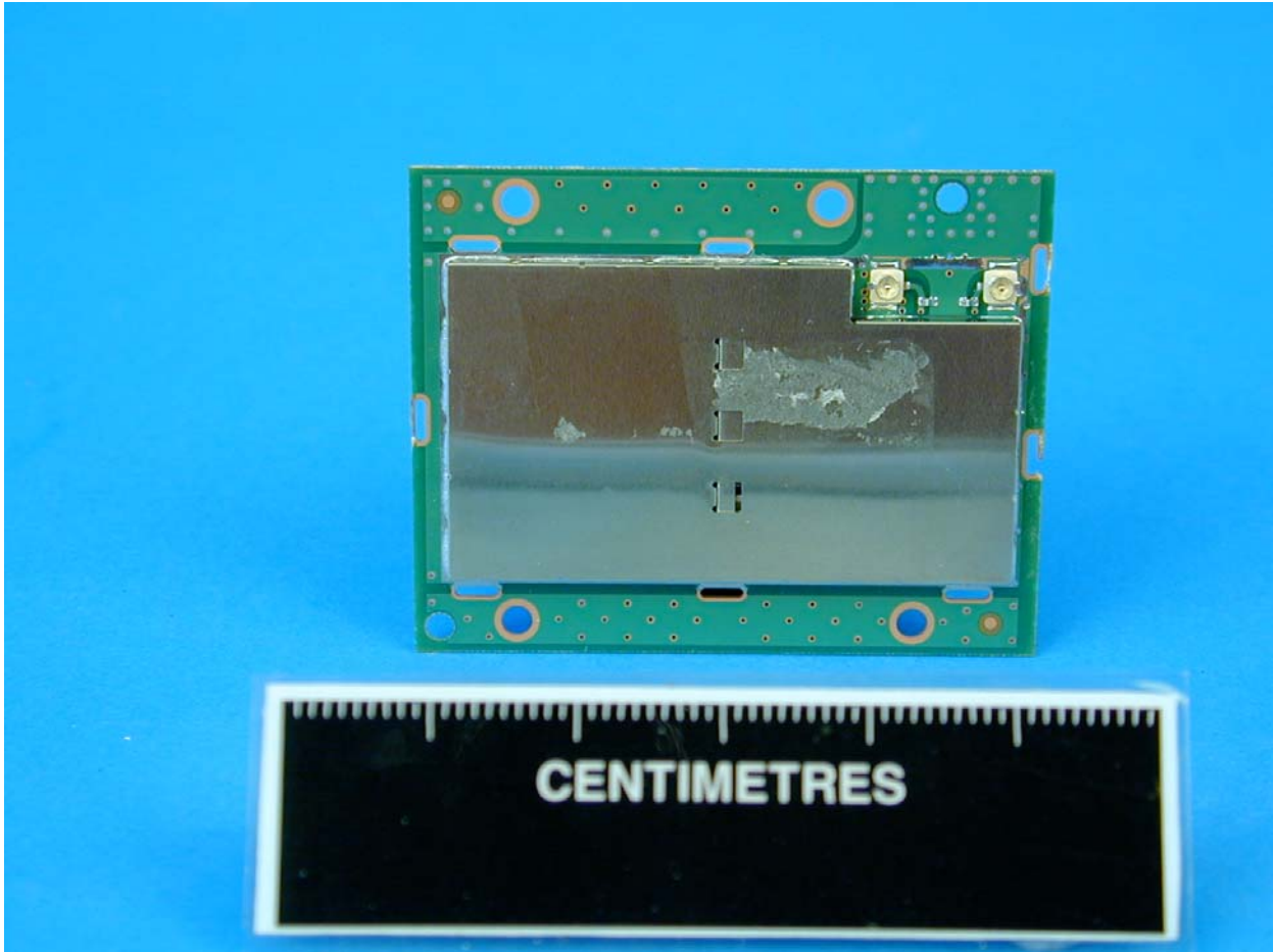
Rear View 21-21160-01
