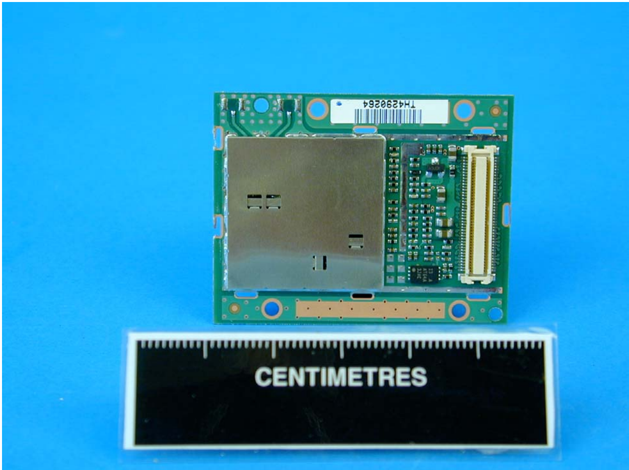
Front View 21-21160-01
