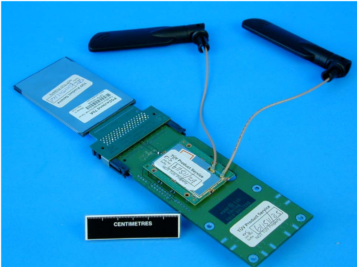
View Showing Extender Cards & Antennas
