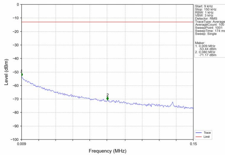
Band66_15MHz_16QAM_HCH_1772.5MHz_RB_1_0_NTNV
