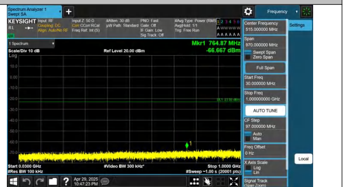
Band66-3MHz-QPSK-131987-1RB#14-30~1000-PASS
