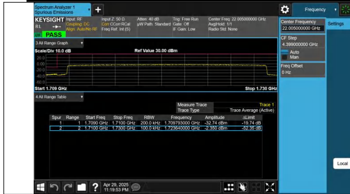
Band66-20MHz-QPSK-132072-100RB#0-PASS
