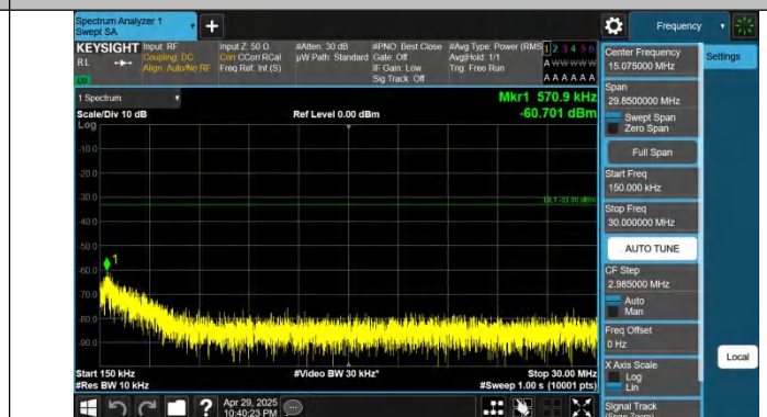
Band66-1.4MHz-QPSK-132665-1RB#0-0.15~30-PASS
