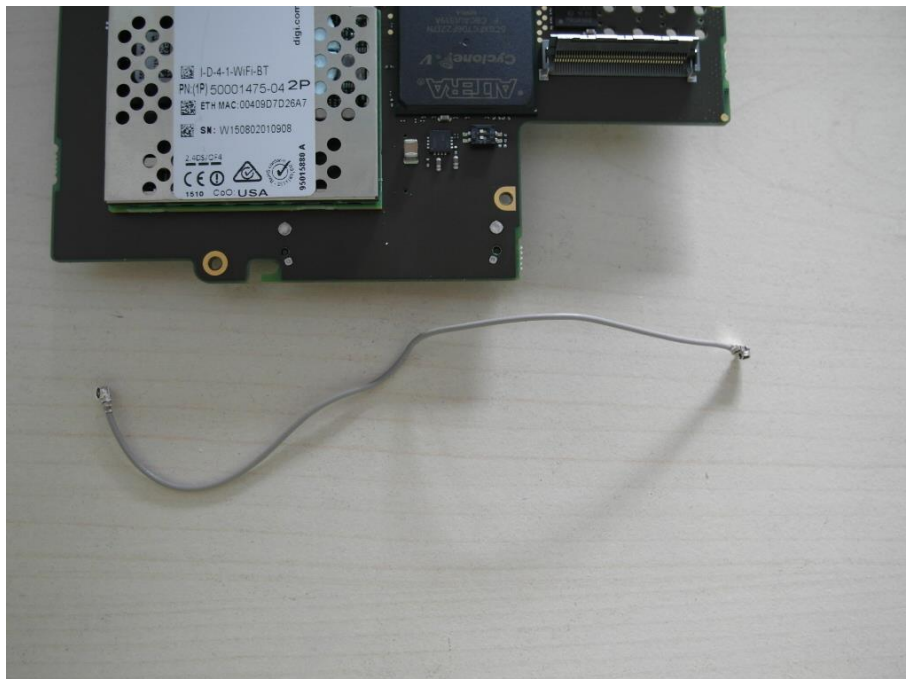
Photo 28: Antenna cable
