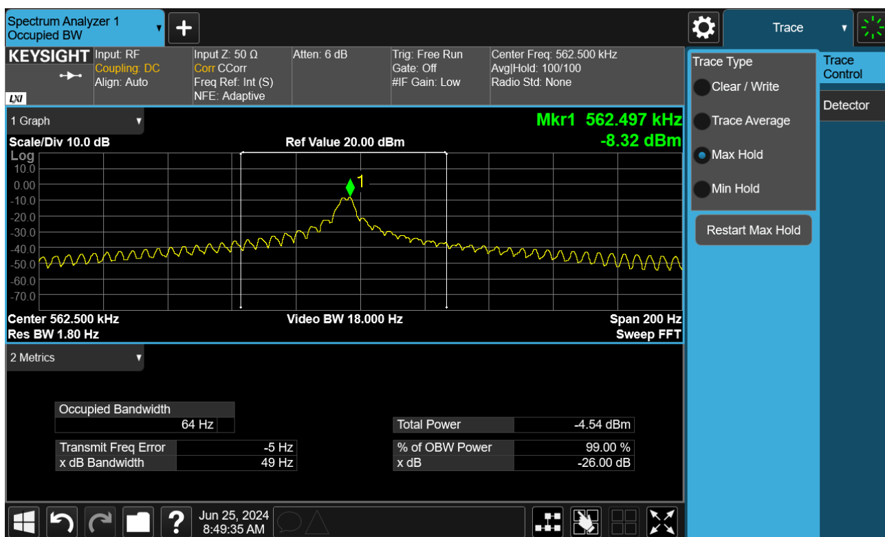
Plot 7-4. Occupied Bandwidth Measurement – Hover
