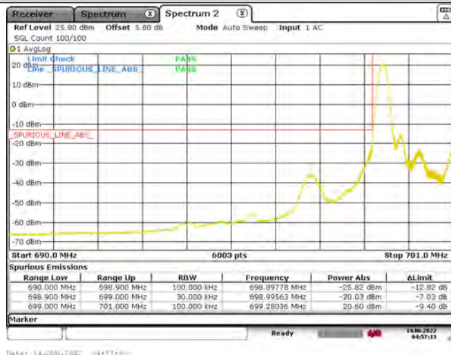
Band12-1.4MHz-QPSK-23017-6RB#0
