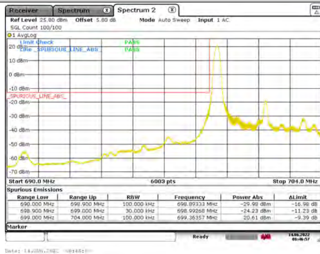
Band12-5MHz-16QAM-23035-25RB#0
