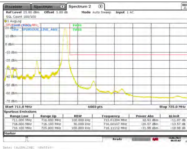
Band12-5MHz-QPSK-23155-25RB#0
