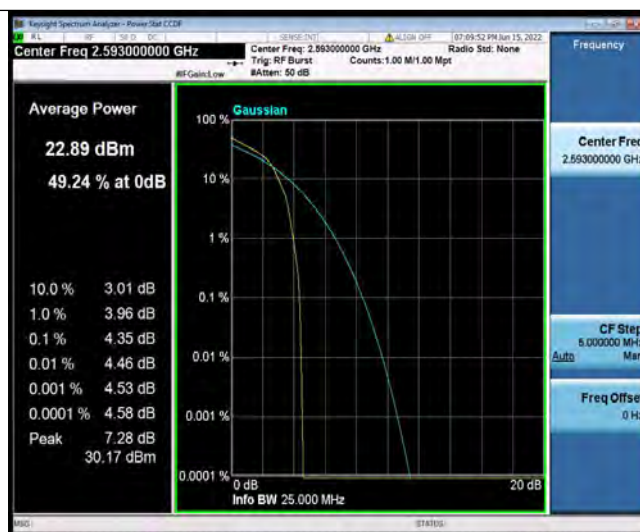
Band41-20MHz-16QAM-40620-27RB#0
