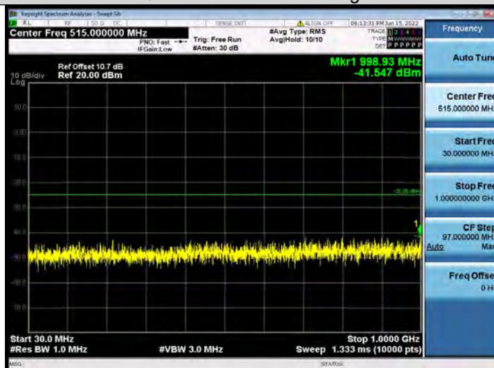
Band41-5MHz-QPSK-40620-1RB#0-Range1:30~1000MHz
