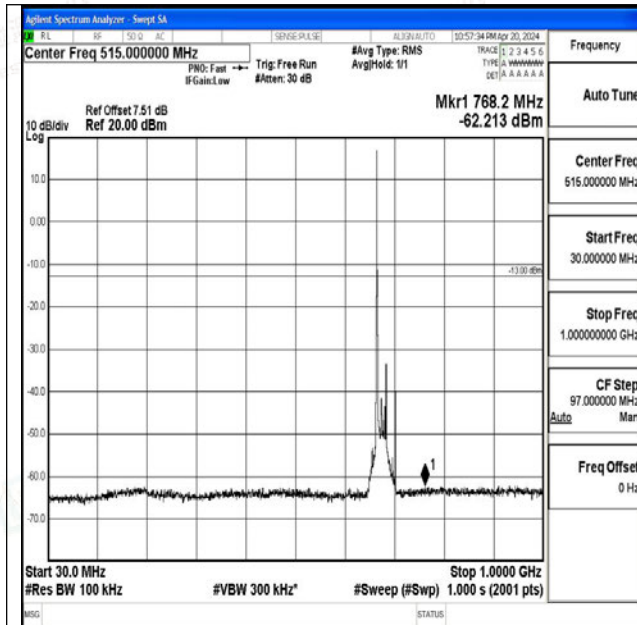
Band71_20MHz_QPSK_133322_1RB#0_30~1000_30~1000
