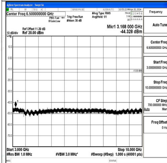
Band71_20MHz_QPSK_133222_1RB#0_3000~10000_3000~10000
