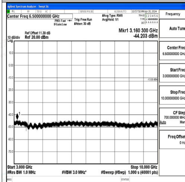
Band71_20MHz_QPSK_133322_1RB#0_3000~10000_3000~10000
