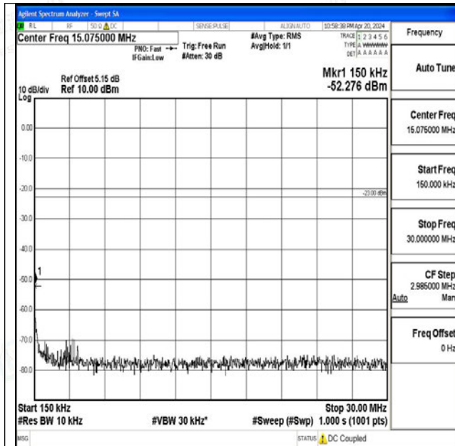
Band71_20MHz_16QAM_133322_1RB#0_0.15~30_0.15 ~30
