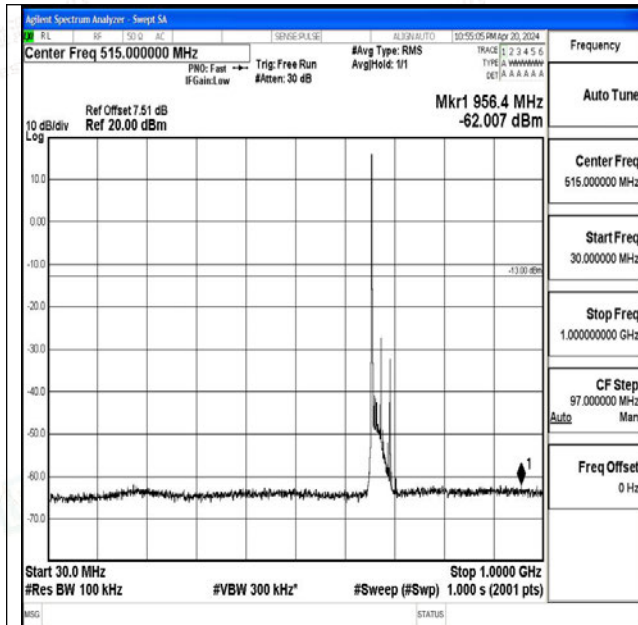
Band71_20MHz_QPSK_133222_1RB#0_30~1000_30~1000
