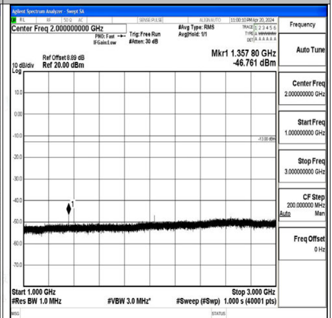
Band71_20MHz_QPSK_133372_1RB#0_1000~3000_10 00~3000
