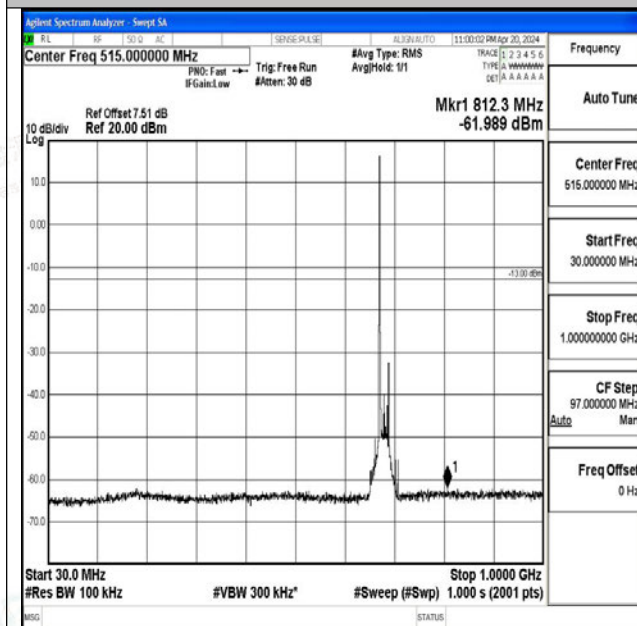
Band71_20MHz_QPSK_133372_1RB#0_30~1000_30~1 000
