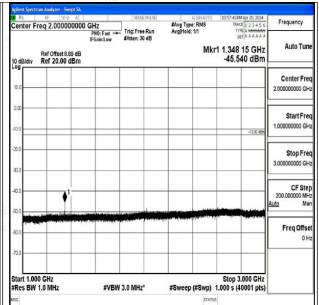
Band71_20MHz_QPSK_133322_1RB#0_1000~3000_1000~3000
