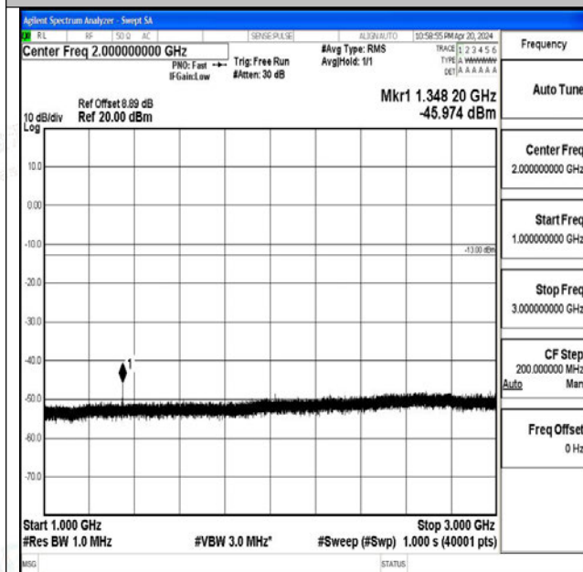
Band71_20MHz_16QAM_133322_1RB#0_1000~3000_1 000~3000
