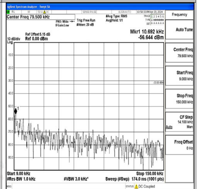
Band71_20MHz_16QAM_133322_1RB#0_0.009~0.15_0.009~0.15
