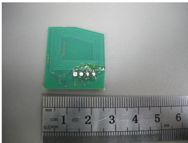
Photograph 7.2.1 Antenna assembly
