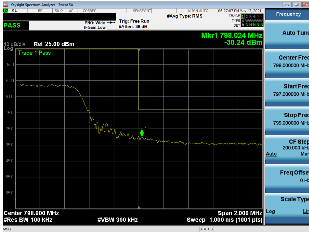
Plot 7-10. Upper Band Edge Plot (LTE Band 14, 10MHz QPSK - RB Size 50)
