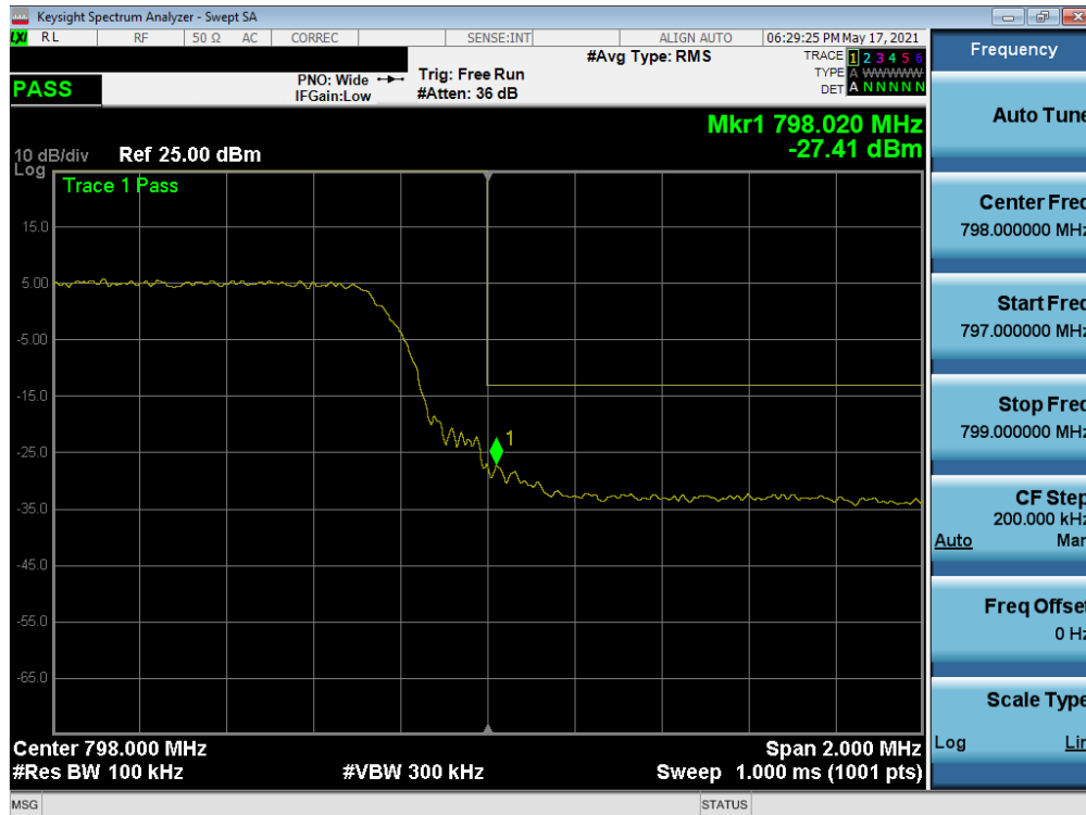
Plot 7-14. Upper Band Edge Plot (LTE Band 14, 5MHz QPSK - RB Size 25)
