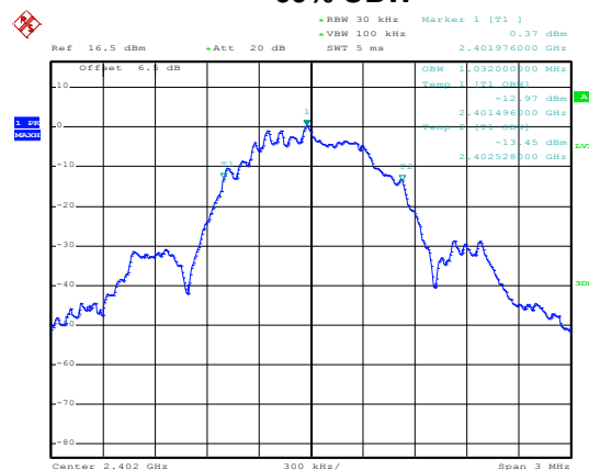
99% OBW
