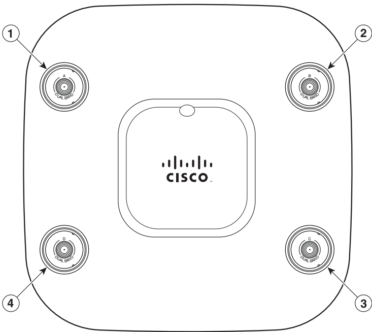
Figure 1 Access Point Ports and Connections (top)—3702P Model
