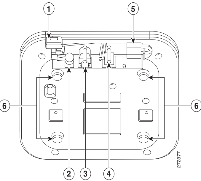
Figure 2 Access Point Ports and Connections (bottom)-AIR3702P
