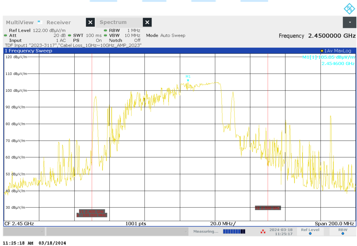
< Fig 10. Frequency Measurements _Load (Minimum Frequency Observed: 2.454 GHz) >
