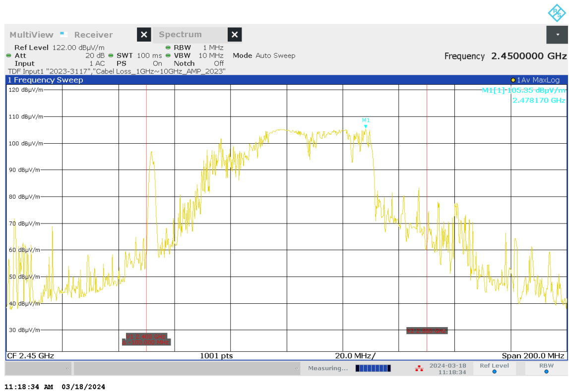
< Fig 9. Frequency Measurements _Load (Maximum Frequency Observed: 2.478 GHz) >
