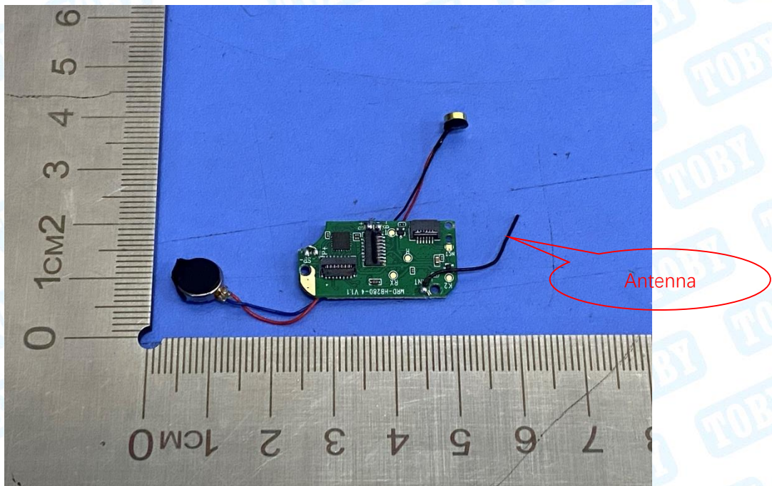
Photo 16 Appearance of PCB
