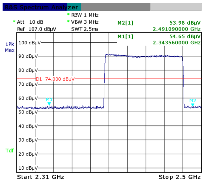
8DPSK hopping-PK
