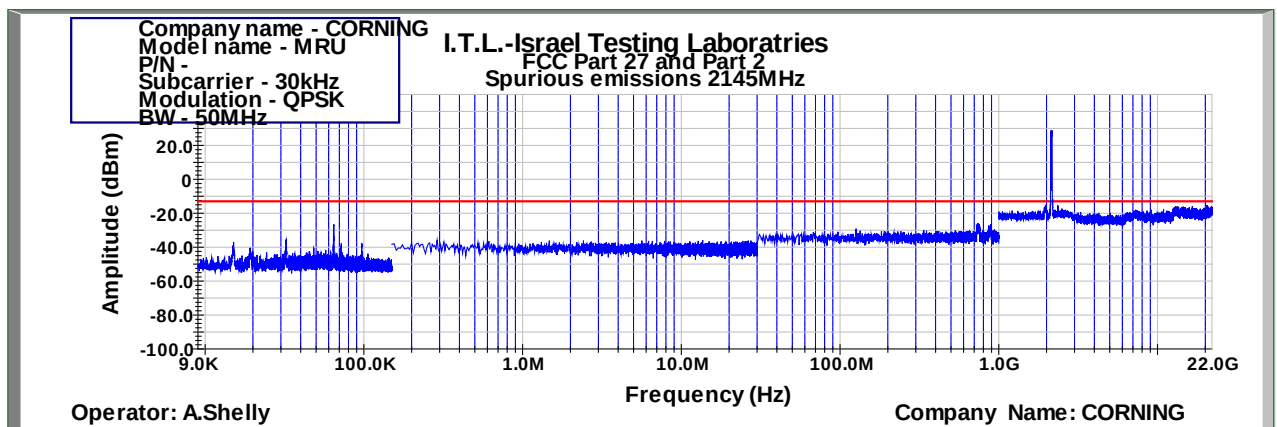
Figure 1054: Spurious Emissions at Antenna Terminal QPSK 50MHz B.W.; 2145.0MHz, 30kHz
