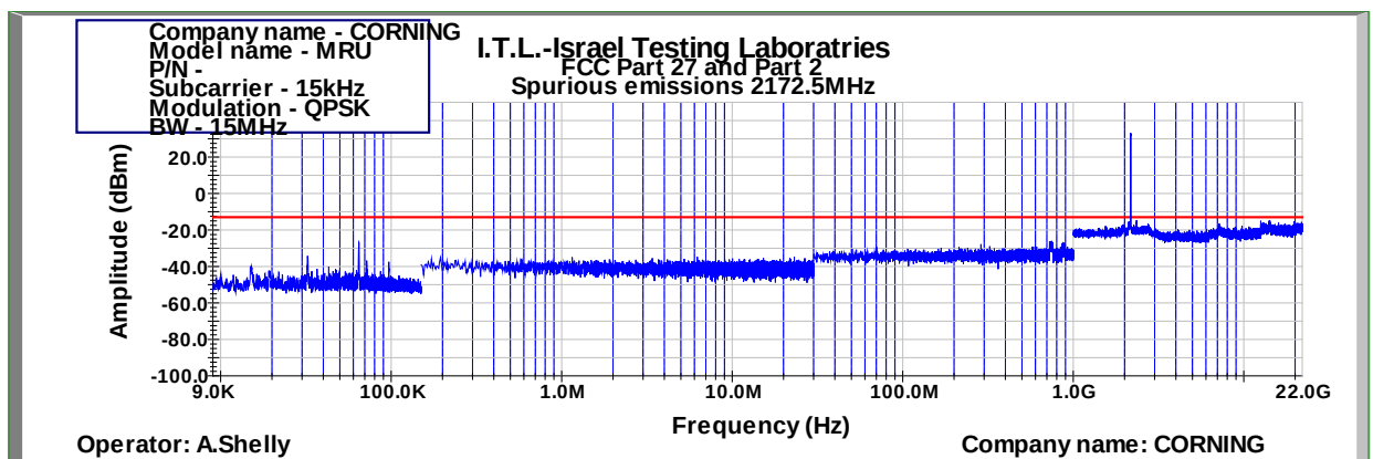
Figure 1016: Spurious Emissions at Antenna Terminal QPSK 15MHz B.W.; 2172.5MHz, 15kHz
