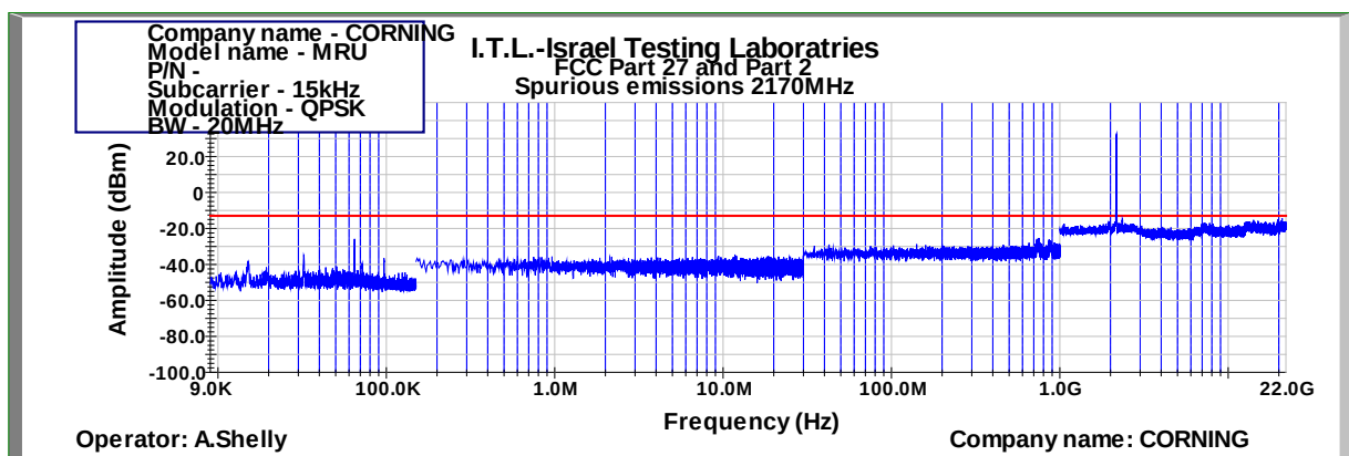
Figure 1025: Spurious Emissions at Antenna Terminal QPSK 20MHz B.W.; 2170.0MHz, 15kHz
