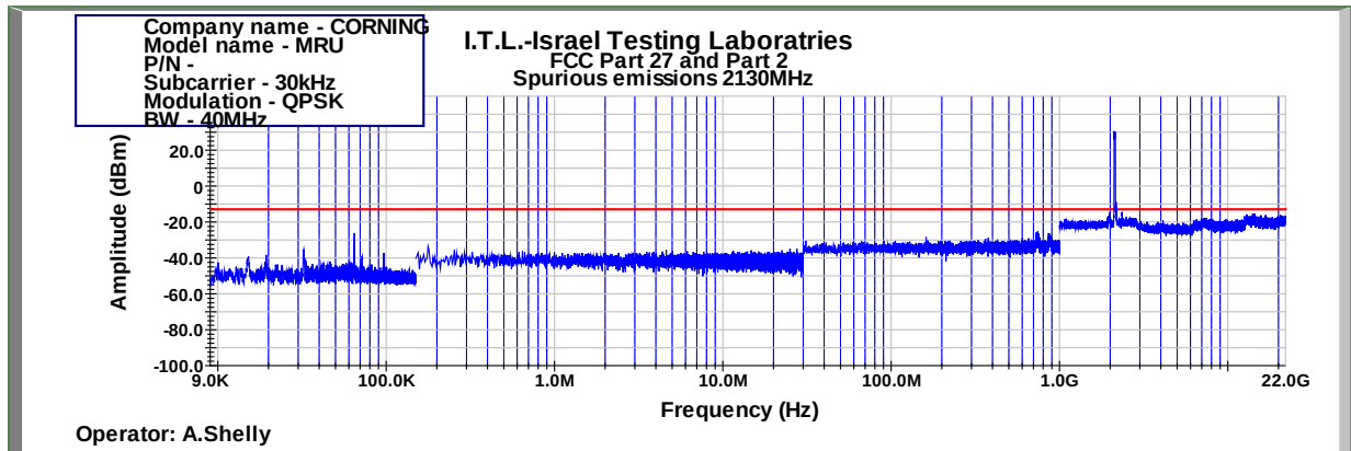
Figure 1044: Spurious Emissions at Antenna Terminal QPSK 40MHz B.W.; 2130.0MHz, 30kHz
