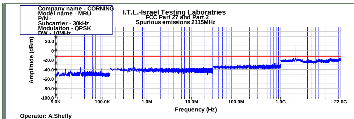
Figure 1008: Spurious Emissions at Antenna Terminal QPSK 10MHz B.W.; 2115.0MHz, 30kHz
