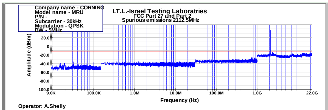
Figure 1002: Spurious Emissions at Antenna Terminal QPSK 5MHz B.W.; 2112.5MHz, 30kHz
