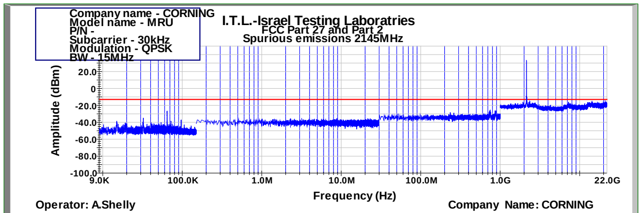
Figure 1018: Spurious Emissions at Antenna Terminal QPSK 15MHz B.W.; 2145.0MHz, 30kHz
