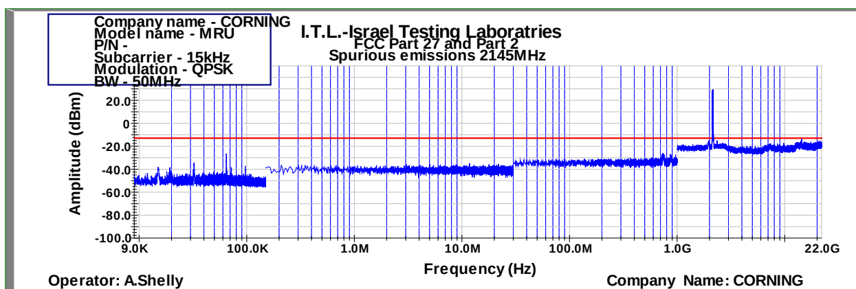
Figure 1051: Spurious Emissions at Antenna Terminal QPSK 50MHz B.W.; 2145.0MHz, 15kHz
