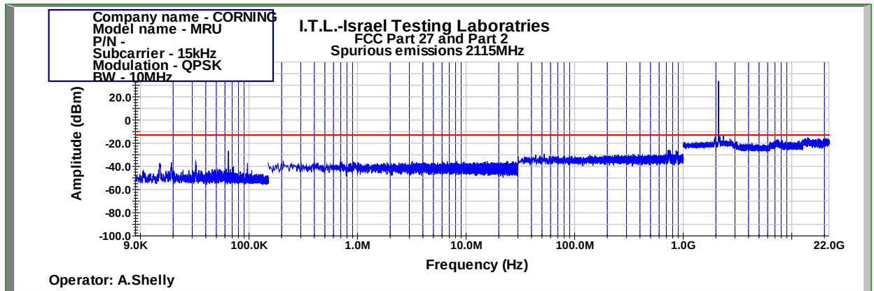
Figure 1005: Spurious Emissions at Antenna Terminal QPSK 10MHz B.W.; 2115.0MHz, 15kHz
