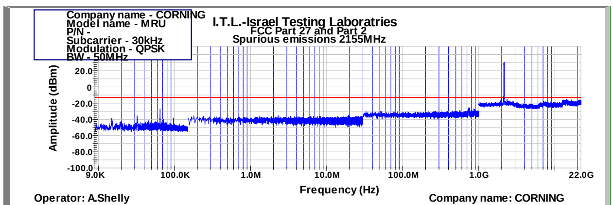
Figure 1055: Spurious Emissions at Antenna Terminal QPSK 50MHz B.W.; 2155.0MHz, 30kHz
