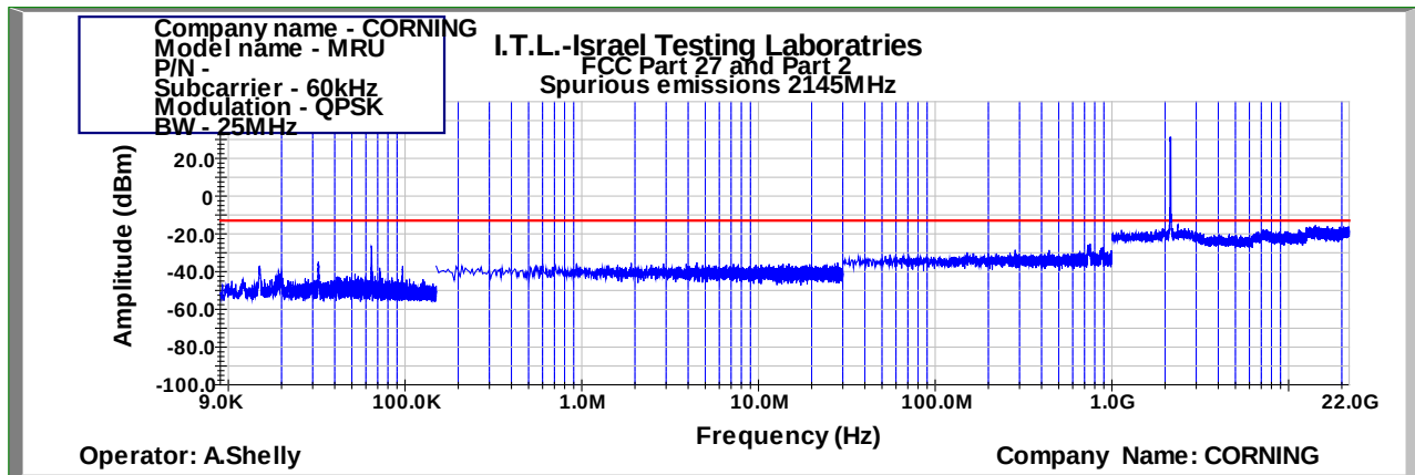
Figure 1039: Spurious Emissions at Antenna Terminal QPSK 25MHz B.W.; 2145.0MHz, 60kHz
