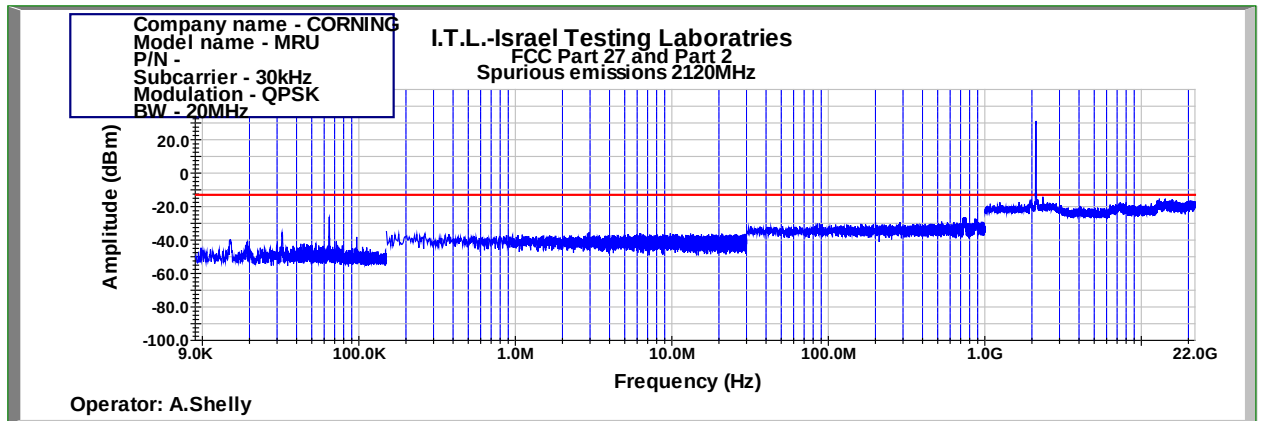
Figure 1026: Spurious Emissions at Antenna Terminal QPSK 20MHz B.W.; 2120.0MHz, 30kHz
