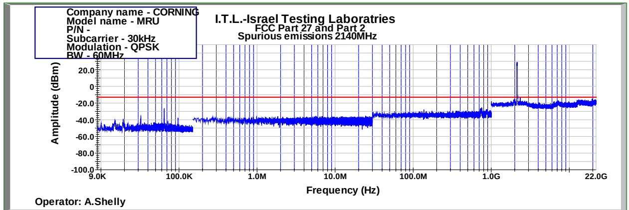
Figure 1059: Spurious Emissions at Antenna Terminal QPSK 60MHz B.W.; 2140.0MHz, 30kHz
