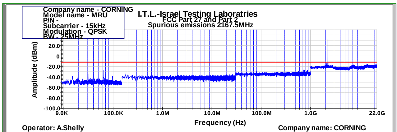
Figure 1034: Spurious Emissions at Antenna Terminal QPSK 25MHz B.W.; 2167.5MHz, 15kHz
