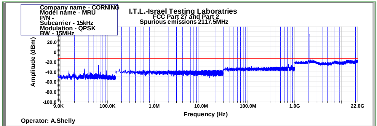
Figure 1014: Spurious Emissions at Antenna Terminal QPSK 15MHz B.W.; 2117.5MHz, 15kHz
