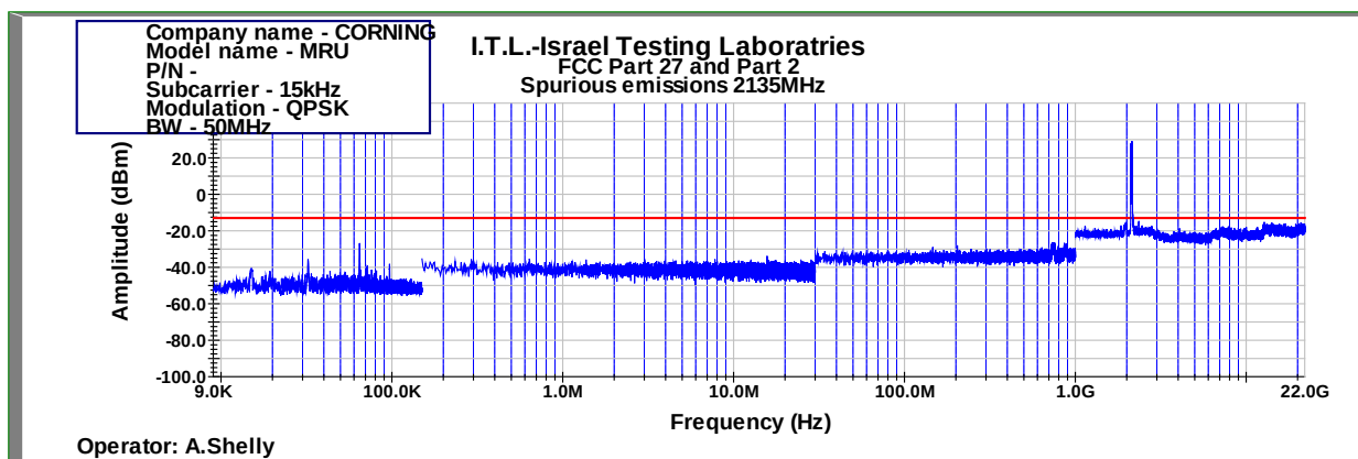
Figure 1050: Spurious Emissions at Antenna Terminal QPSK 50MHz B.W.; 2135.0MHz, 15kHz
