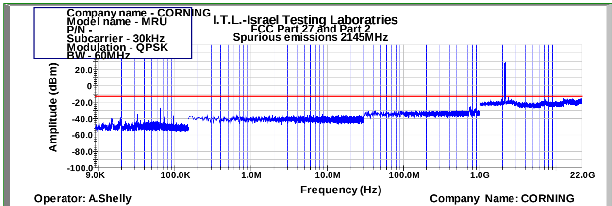
Figure 1060: Spurious Emissions at Antenna Terminal QPSK 60MHz B.W.; 2145.0MHz, 30kHz
