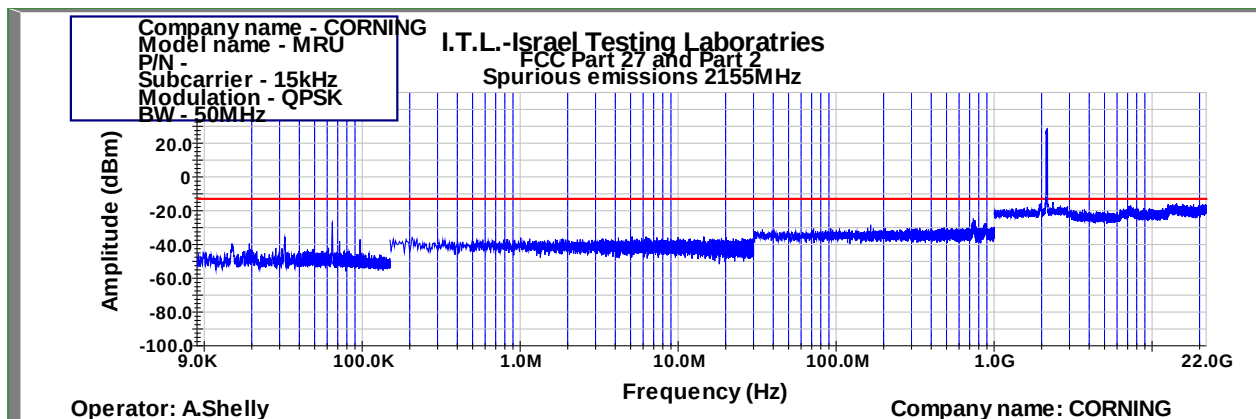
Figure 1052: Spurious Emissions at Antenna Terminal QPSK 50MHz B.W.; 2155.0MHz, 15kHz
