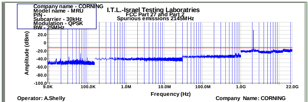
Figure 1036: Spurious Emissions at Antenna Terminal QPSK 25MHz B.W.; 2145.0MHz, 30kHz
