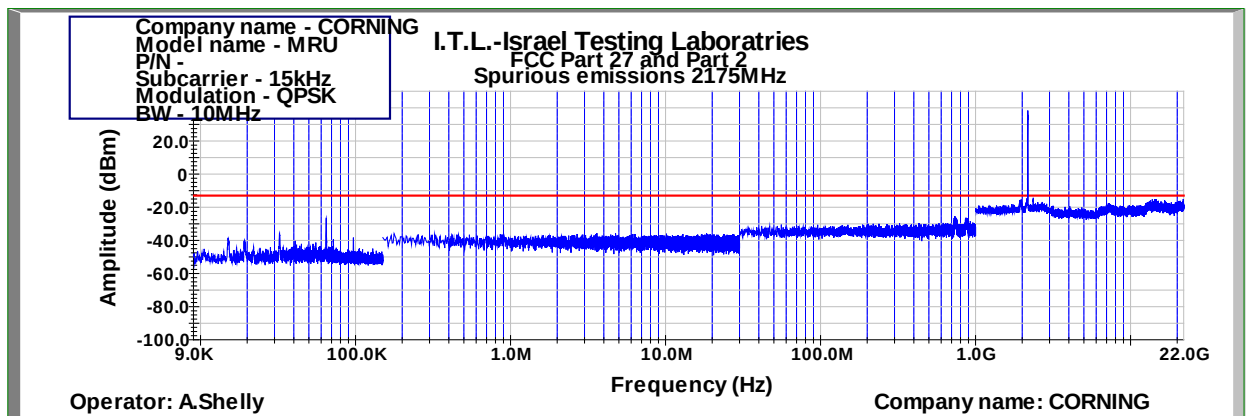
Figure 1007: Spurious Emissions at Antenna Terminal QPSK 10MHz B.W.; 2175.0MHz, 15kHz
