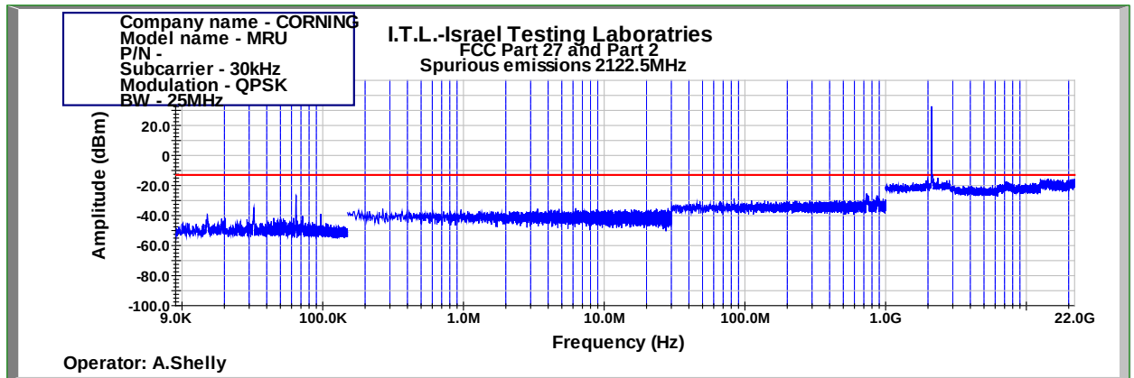
Figure 1035: Spurious Emissions at Antenna Terminal QPSK 25MHz B.W.; 2122.5MHz, 30kHz
