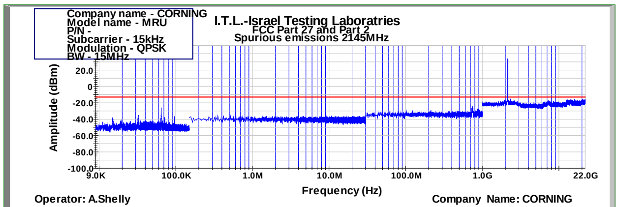
Figure 1015: Spurious Emissions at Antenna Terminal QPSK 15MHz B.W.; 2145.0MHz, 15kHz
