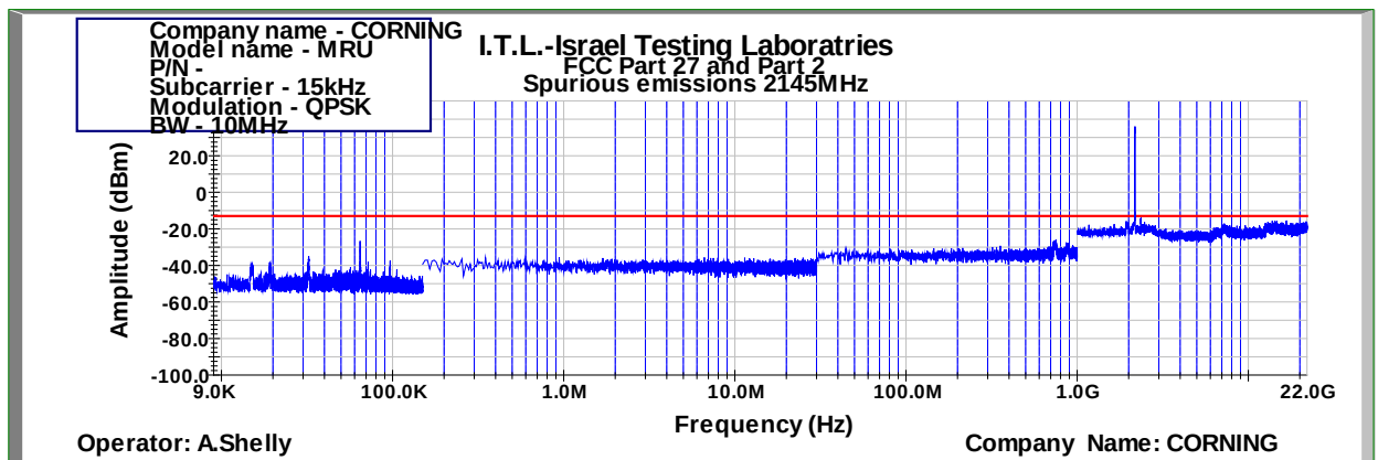
Figure 1006: Spurious Emissions at Antenna Terminal QPSK 10MHz B.W.; 2145.0MHz, 15kHz
