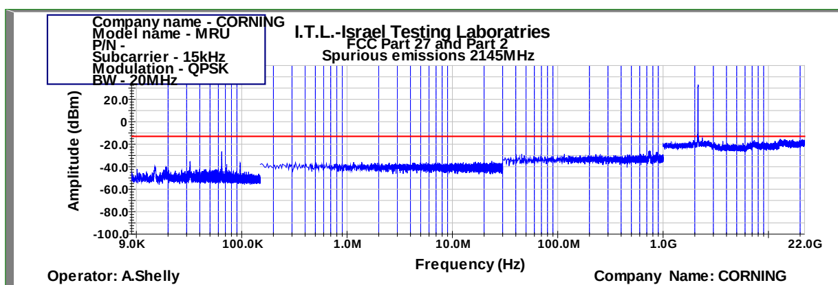
Figure 1024: Spurious Emissions at Antenna Terminal QPSK 20MHz B.W.; 2145.0MHz, 15kHz
