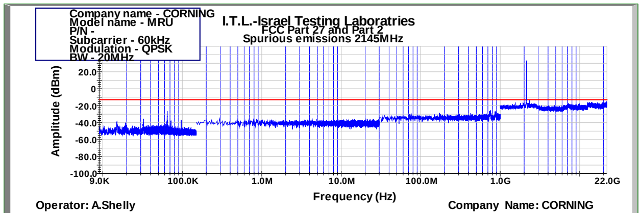
Figure 1030: Spurious Emissions at Antenna Terminal QPSK 20MHz B.W.; 2145.0MHz, 60kHz
