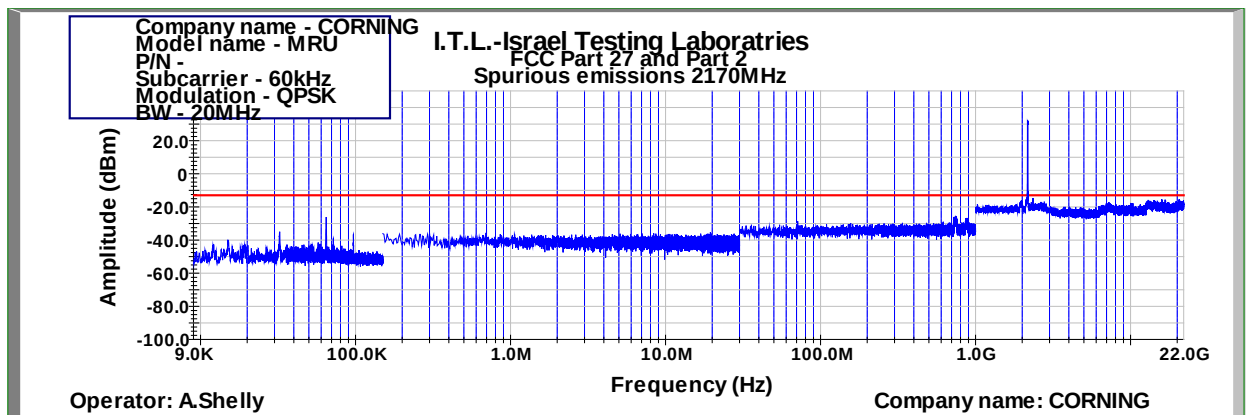
Figure 1031: Spurious Emissions at Antenna Terminal QPSK 20MHz B.W.; 2170.0MHz, 60kHz
