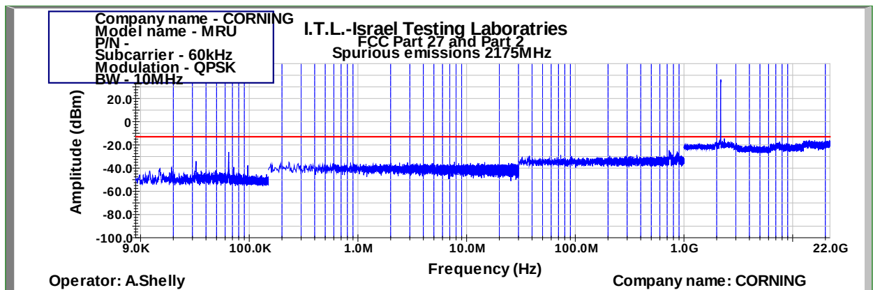
Figure 1013: Spurious Emissions at Antenna Terminal QPSK 10MHz B.W.; 2175.0MHz, 60kHz
