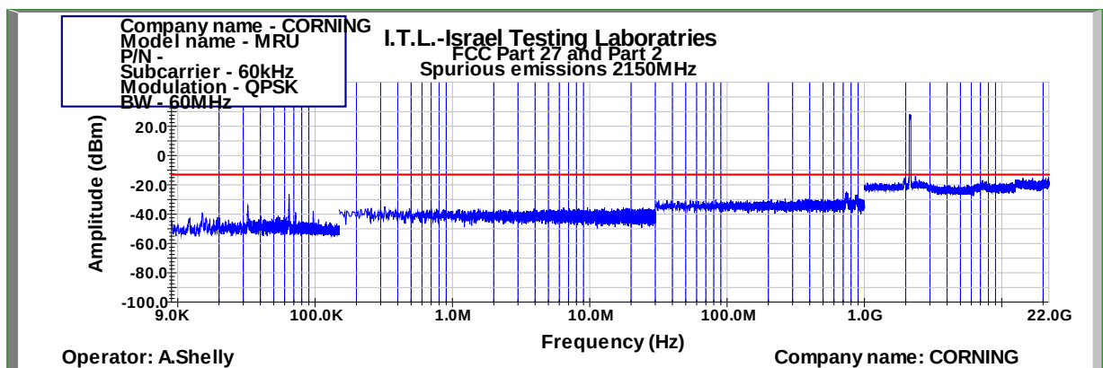
Figure 1064: Spurious Emissions at Antenna Terminal QPSK 60MHz B.W.; 2150.0MHz, 60kHz
