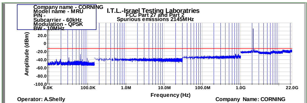
Figure 1012: Spurious Emissions at Antenna Terminal QPSK 10MHz B.W.; 2145.0MHz, 60kHz
