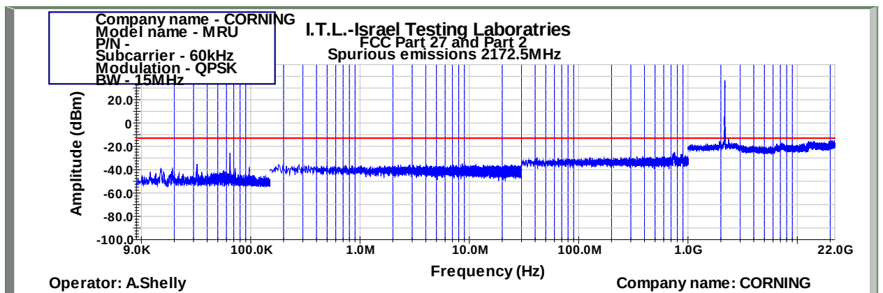
Figure 1022: Spurious Emissions at Antenna Terminal QPSK 15MHz B.W.; 2172.5MHz, 60kHz
