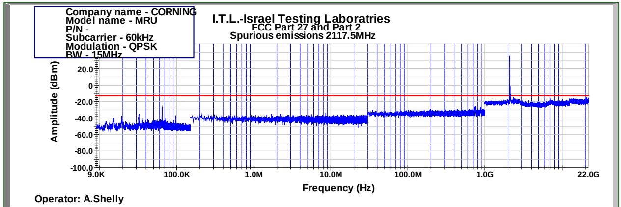
Figure 1020: Spurious Emissions at Antenna Terminal QPSK 15MHz B.W.; 2117.5MHz, 60kHz
