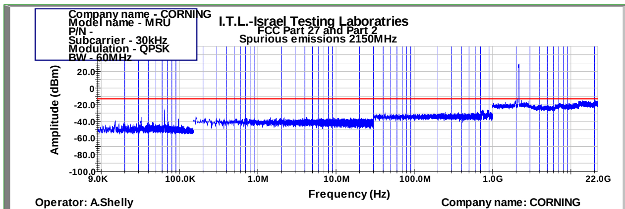
Figure 1061: Spurious Emissions at Antenna Terminal QPSK 60MHz B.W.; 2150.0MHz, 30kHz
