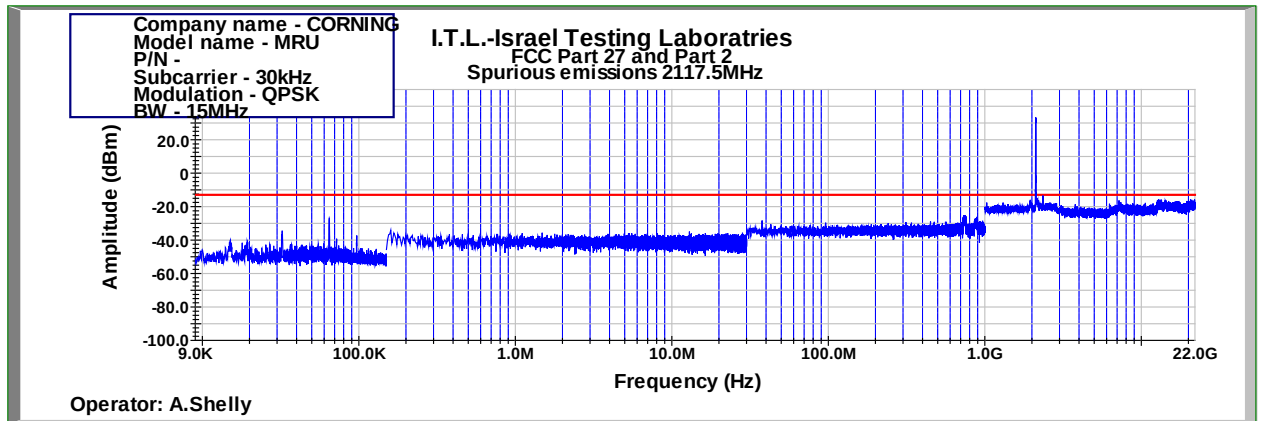
Figure 1017: Spurious Emissions at Antenna Terminal QPSK 15MHz B.W.; 2117.5MHz, 30kHz
