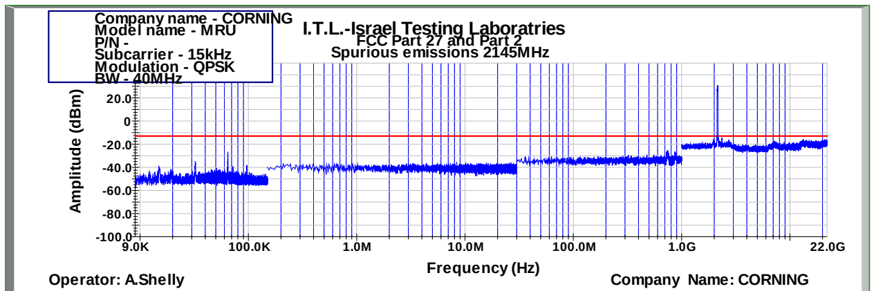
Figure 1042: Spurious Emissions at Antenna Terminal QPSK 40MHz B.W.; 2145.0MHz, 15kHz
