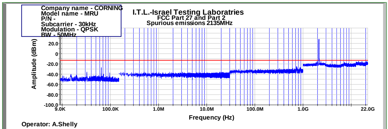
Figure 1053: Spurious Emissions at Antenna Terminal QPSK 50MHz B.W.; 2135.0MHz, 30kHz
