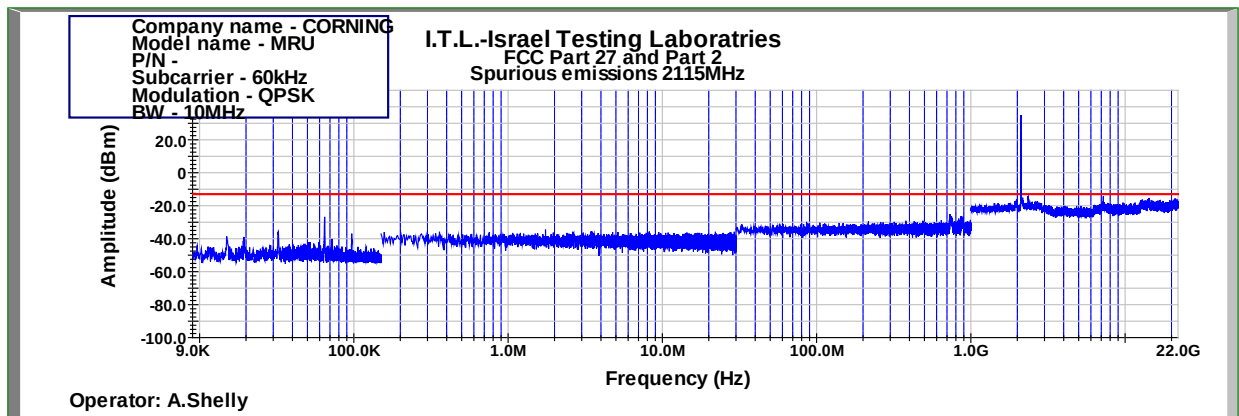
Figure 1011: Spurious Emissions at Antenna Terminal QPSK 10MHz B.W.; 2115.0MHz, 60kHz
