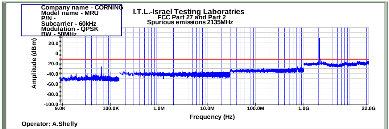
Figure 1056: Spurious Emissions at Antenna Terminal QPSK 50MHz B.W.; 2135.0MHz, 60kHz
