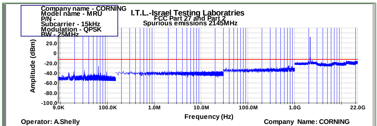
Figure 1033: Spurious Emissions at Antenna Terminal QPSK 25MHz B.W.; 2145.0MHz, 15kHz
