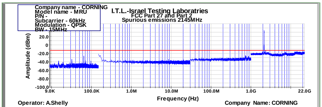
Figure 1021: Spurious Emissions at Antenna Terminal QPSK 15MHz B.W.; 2145.0MHz, 60kHz
