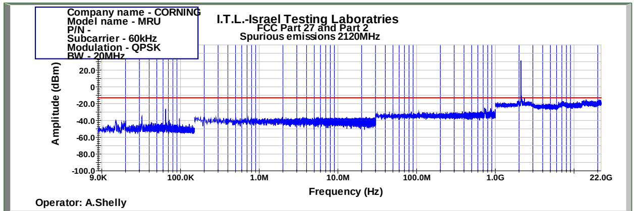
Figure 1029: Spurious Emissions at Antenna Terminal QPSK 20MHz B.W.; 2120.0MHz, 60kHz
