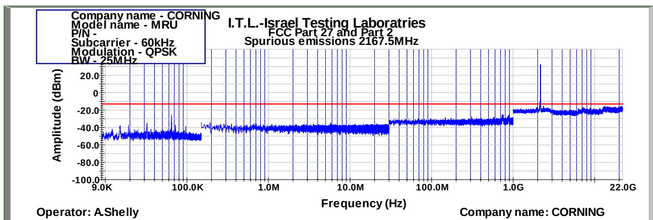
Figure 1040: Spurious Emissions at Antenna Terminal QPSK 25MHz B.W.; 2167.5MHz, 60kHz
