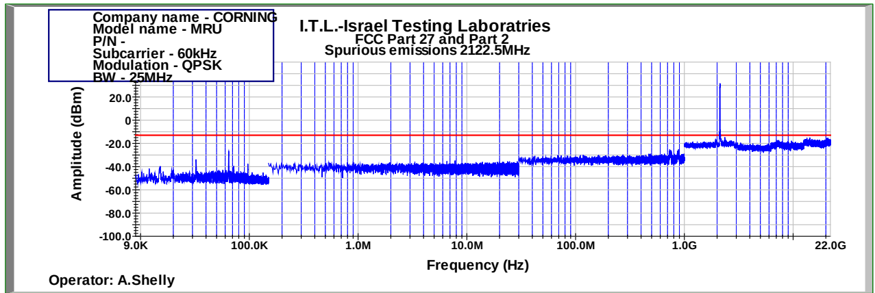
Figure 1038: Spurious Emissions at Antenna Terminal QPSK 25MHz B.W.; 2122.5MHz, 60kHz
