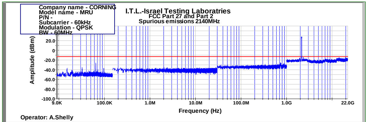
Figure 1062: Spurious Emissions at Antenna Terminal QPSK 60MHz B.W.; 2140.0MHz, 60kHz
