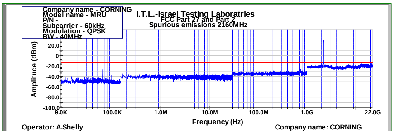
Figure 1049: Spurious Emissions at Antenna Terminal QPSK 40MHz B.W.; 2160.0MHz, 60kHz
