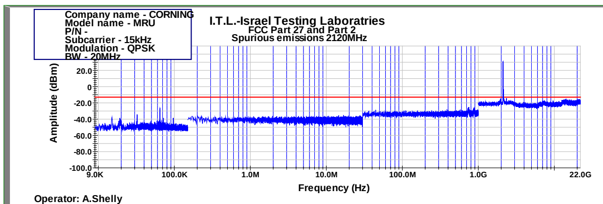
Figure 1023: Spurious Emissions at Antenna Terminal QPSK 20MHz B.W.; 2120.0MHz, 15kHz
