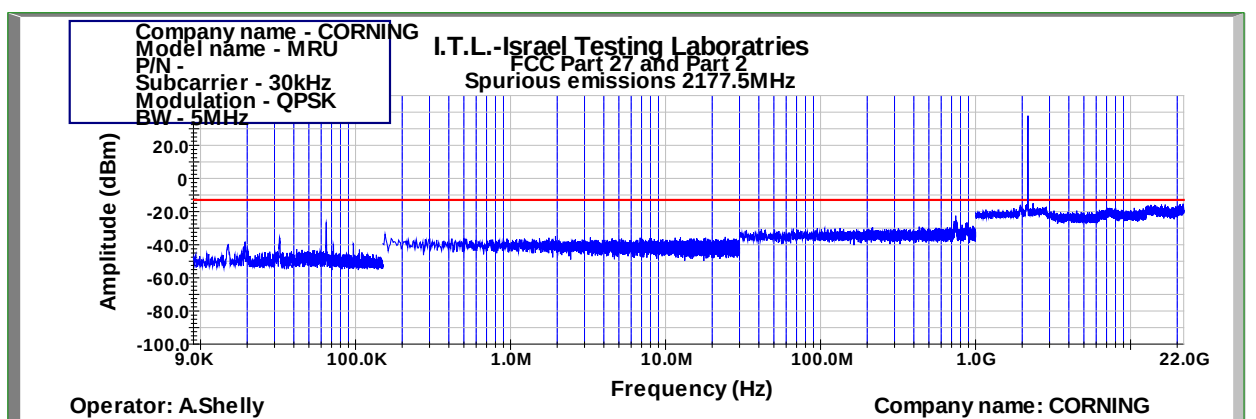
Figure 1004: Spurious Emissions at Antenna Terminal QPSK 5MHz B.W.; 2177.5MHz, 30kHz
