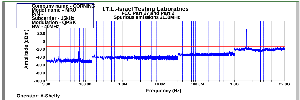
Figure 1041: Spurious Emissions at Antenna Terminal QPSK 40MHz B.W.; 2130.0MHz, 15kHz
