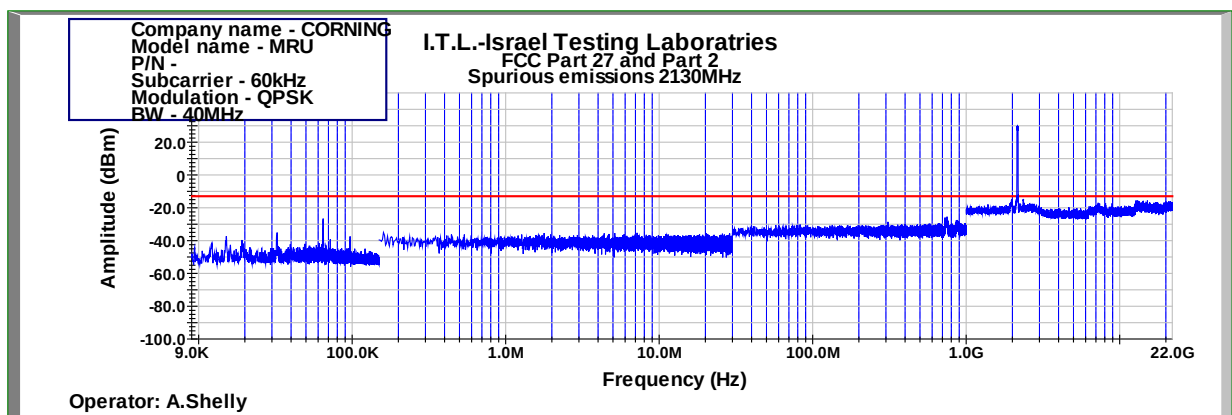
Figure 1047: Spurious Emissions at Antenna Terminal QPSK 40MHz B.W.; 2130.0MHz, 60kHz
