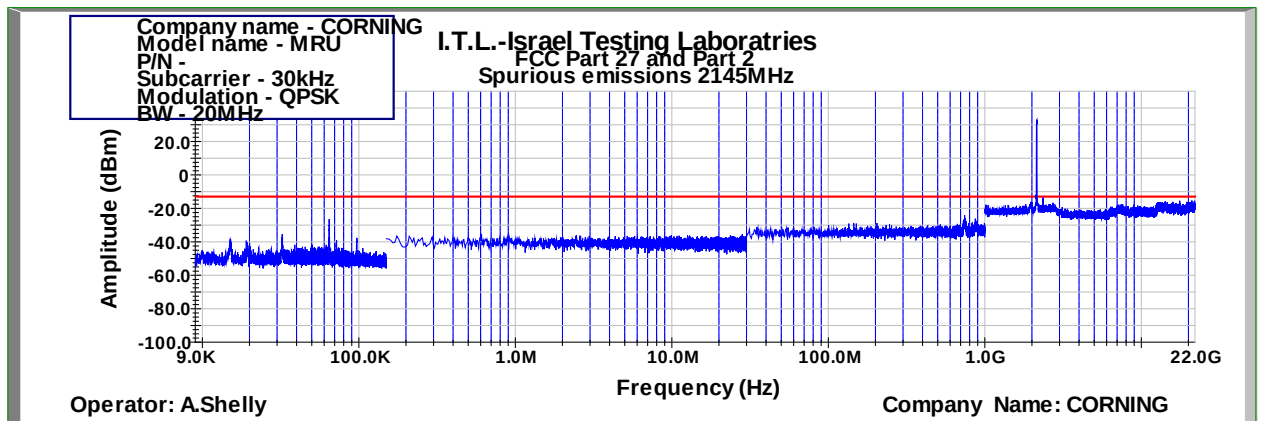
Figure 1027: Spurious Emissions at Antenna Terminal QPSK 20MHz B.W.; 2145.0MHz, 30kHz
