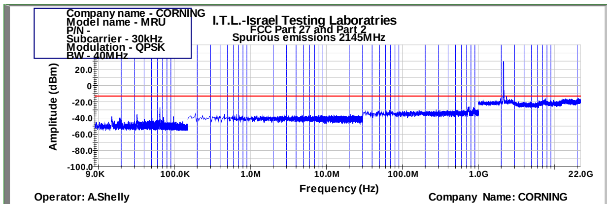
Figure 1045: Spurious Emissions at Antenna Terminal QPSK 40MHz B.W.; 2145.0MHz, 30kHz
