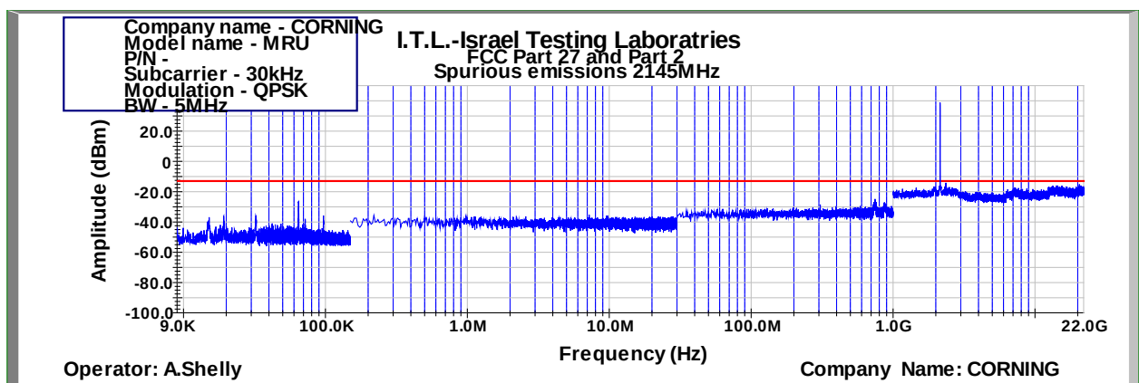
Figure 1003: Spurious Emissions at Antenna Terminal QPSK 5MHz B.W.; 2145.0MHz, 30kHz
