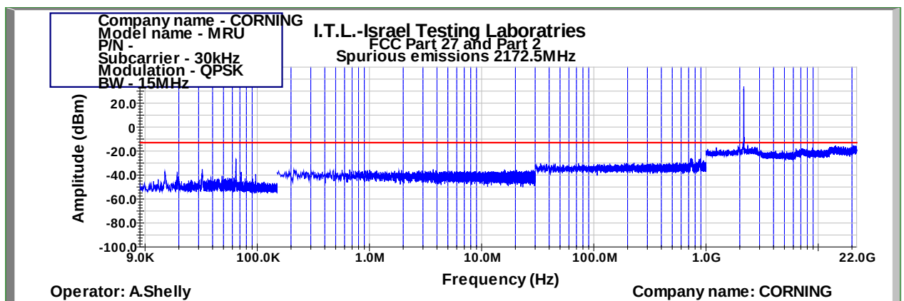
Figure 1019: Spurious Emissions at Antenna Terminal QPSK 15MHz B.W.; 2172.5MHz, 30kHz
