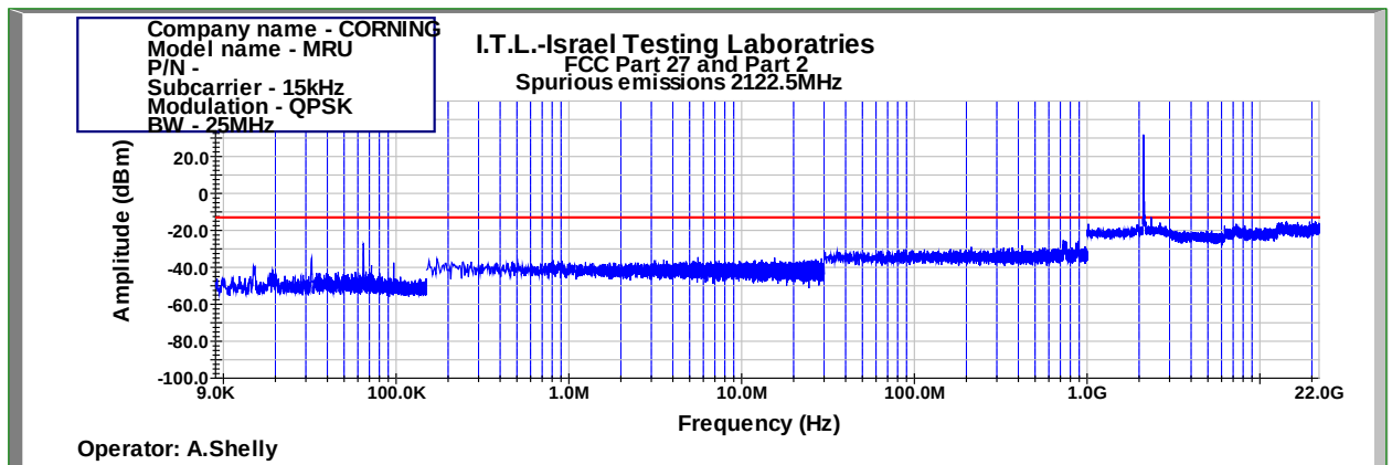
Figure 1032: Spurious Emissions at Antenna Terminal QPSK 25MHz B.W.; 2122.5MHz, 15kHz
