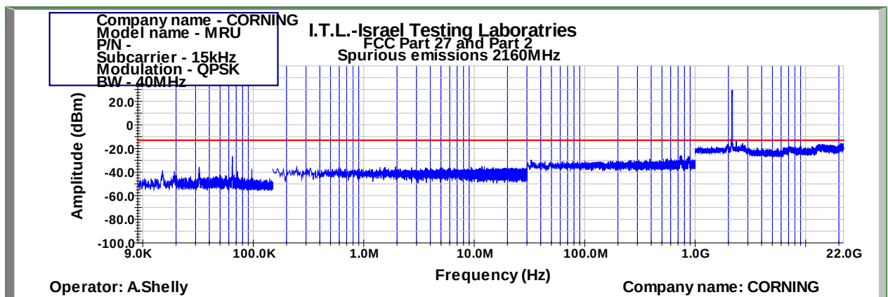
Figure 1043: Spurious Emissions at Antenna Terminal QPSK 40MHz B.W.; 2160.0MHz, 15kHz
