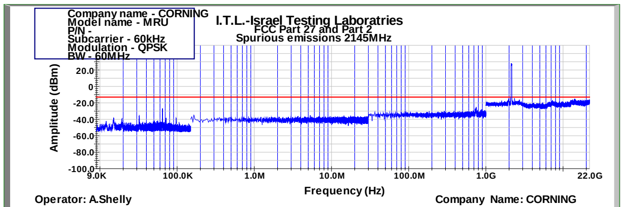
Figure 1063: Spurious Emissions at Antenna Terminal QPSK 60MHz B.W.; 2145.0MHz, 60kHz
