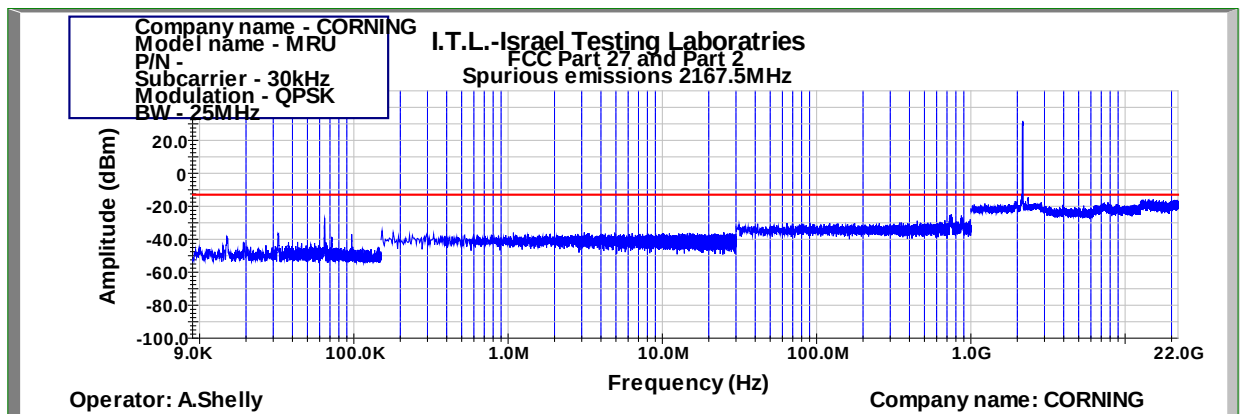
Figure 1037: Spurious Emissions at Antenna Terminal QPSK 25MHz B.W.; 2167.5MHz, 30kHz
