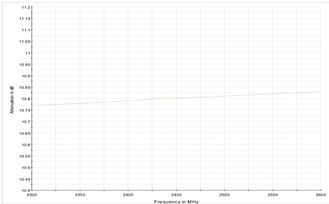
Path attenuation
