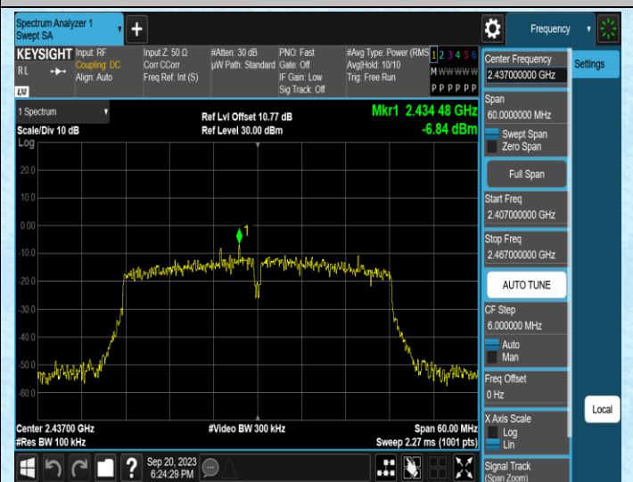
11N40SISO-Ant0-2437-0~Reference
