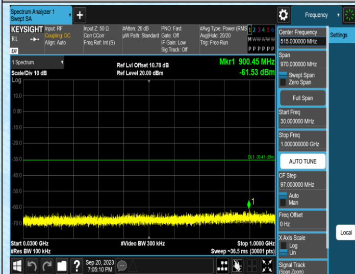
11N40MIMO-Ant1-2422-30~1000
