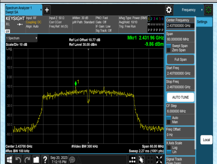
11N40MIMO-Ant1-2437-0-Reference
