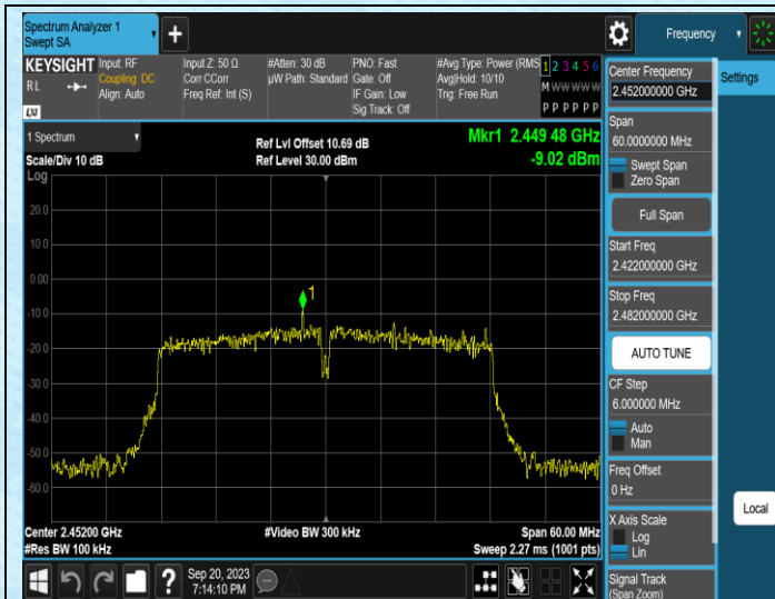
11N40MIMO-Ant0-2452-0-Reference
