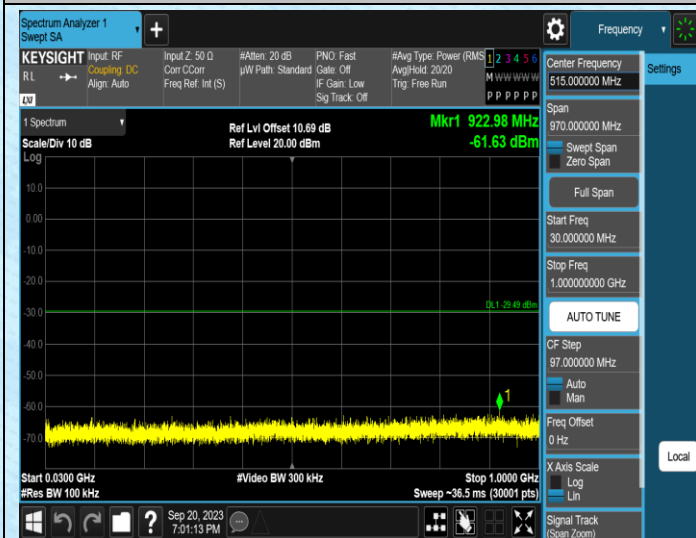
11N20MIMO-Ant1-2462-30~1000
