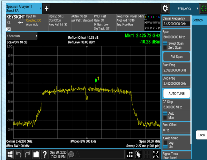
11N40MIMO-Ant0-2422-0-Reference
