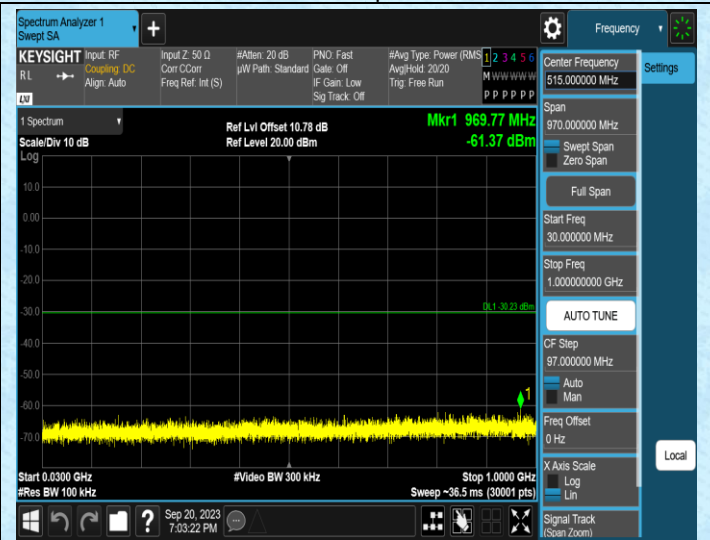
11N40MIMO-Ant0-2422-30~1000
