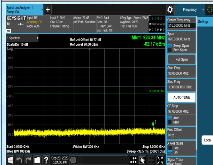
11N40SISO-Ant0-2437-30~1000
