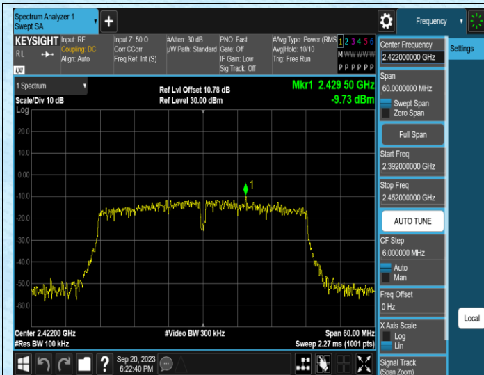
11N40SISO-Ant0-2422-0~Reference
