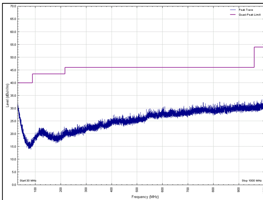
Figure 56 - 30 MHz to 1 GHz, 2437 MHz, Vertical, EUT Orientation X
