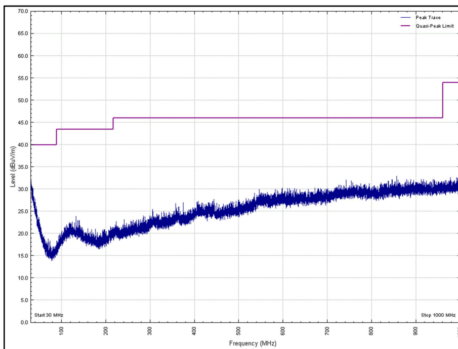
Figure 57 - 30 MHz to 1 GHz, 2437 MHz, Horizontal, EUT Orientation X
