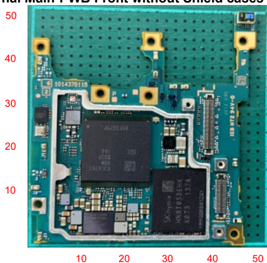
Internal Main-PWB Front without Shield cases (Front-side)
