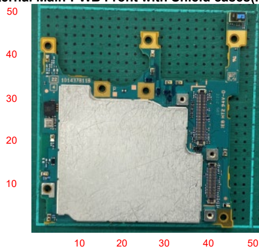
Internal Main-PWB Front with Shield cases(Front-side)
