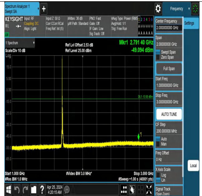
Band66_10MHz_QPSK_132022_1RB#0_1000~3000_1000~3000
