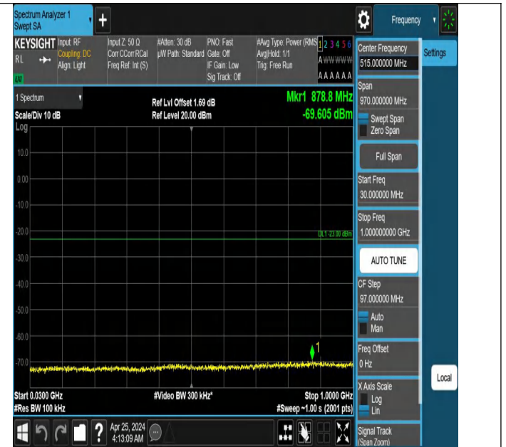
Band66_5MHz_QPSK_132322_1RB#24_30~1000_30~1000
