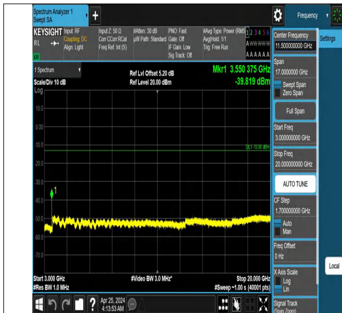
Band66_5MHz_QPSK_132647_1RB#0_3000~20000_3000~2000
