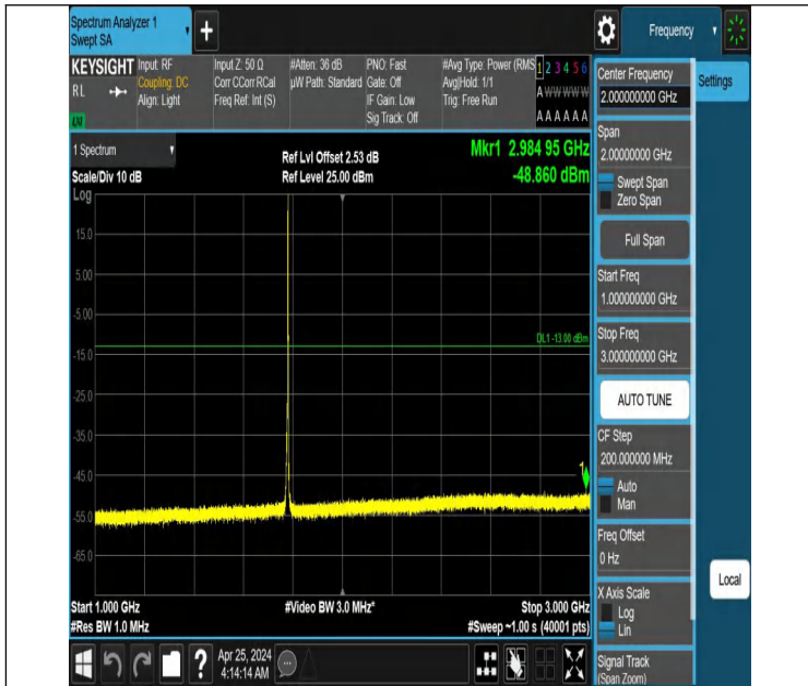
Band66_5MHz_QPSK_132647_1RB#24_1000~3000_1000~3000
