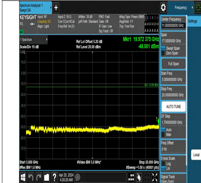
Band66_10MHz_QPSK_132022_1RB#0_3000~20000_3000~200
