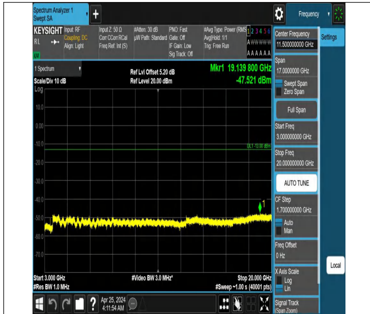
Band66_5MHz_QPSK_131997_1RB#0_3000~20000_3000~2000
