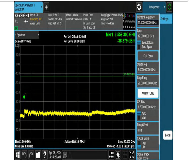
Band66_5MHz_QPSK_132647_1RB#24_3000~20000_3000~2000 0
