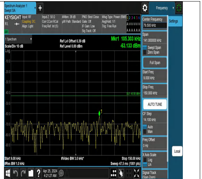
Band66_10MHz_QPSK_132322_1RB#49_0.009~0.15_0.009~0.15
