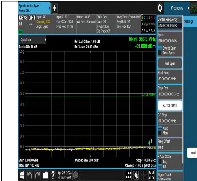
Band66_5MHz_QPSK_132322_1RB#0_30~1000_30~1000
