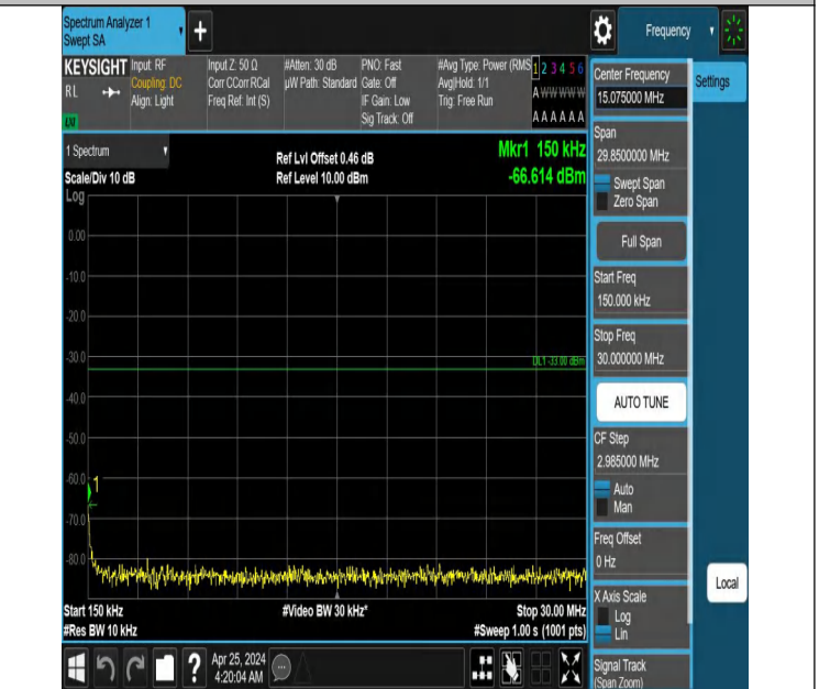
Band66_10MHz_QPSK_132022_1RB#0_0.15~30_0.15~30
