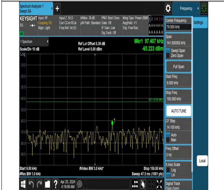
Band66_10MHz_QPSK_132022_1RB#0_0.009~0.15_0.009~0.15
