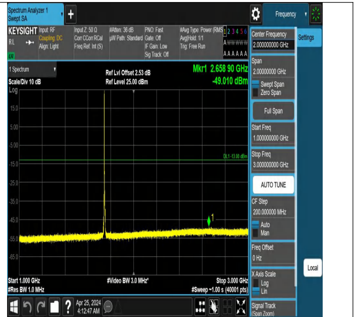
Band66_5MHz_QPSK_132322_1RB#0_1000~3000_1000~3000
