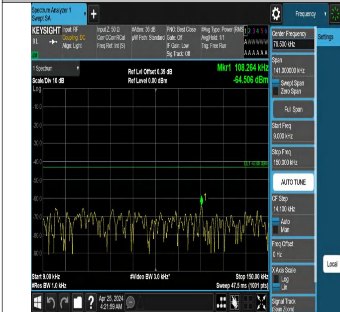
Band66_10MHz_QPSK_132622_1RB#0_0.009~0.15_0.009~0.15
