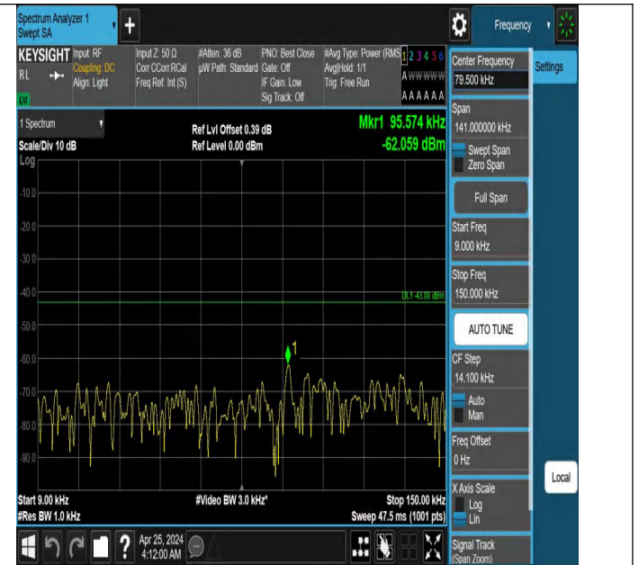
Band66_5MHz_QPSK_131997_1RB#24_0.009~0.15_0.009~0.15
