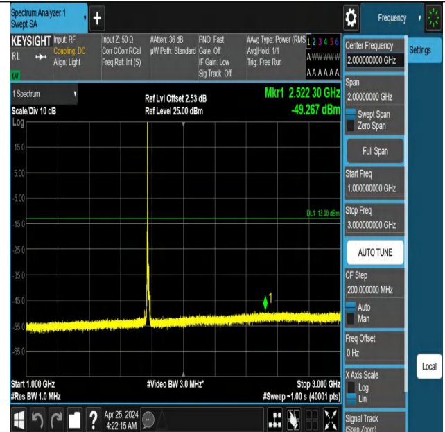
Band66_10MHz_QPSK_132622_1RB#0_1000~3000_1000~3000
