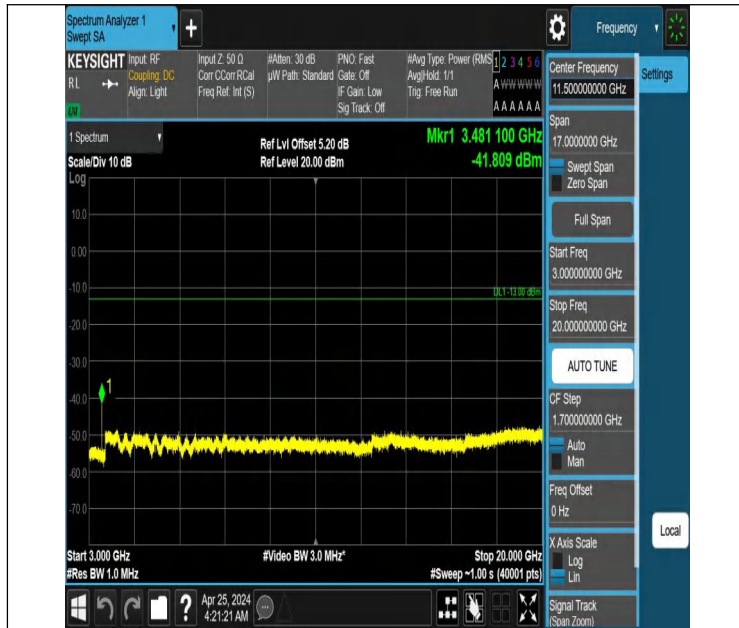
Band66_10MHz_QPSK_132322_1RB#0_3000~20000_3000~20000
