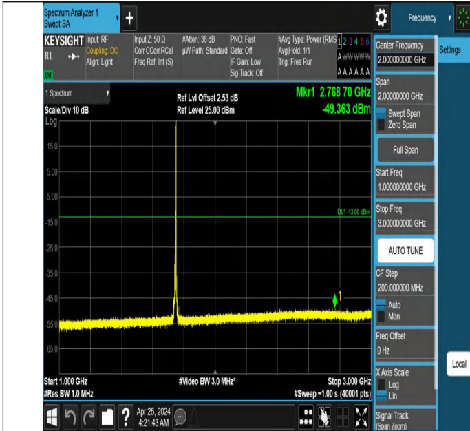
Band66_10MHz_QPSK_132322_1RB#49_1000~3000_1000~300
