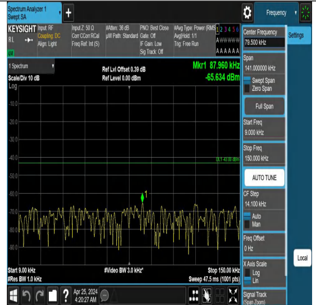
Band66_10MHz_QPSK_132022_1RB#49_0.009~0.15_0.009~0.15
