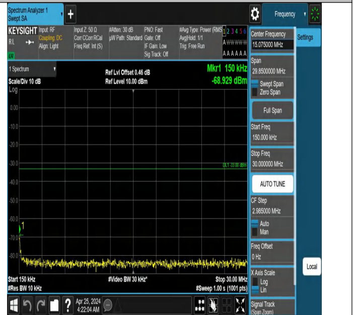
Band66_10MHz_QPSK_132622_1RB#0_0.15~30_0.15~30
