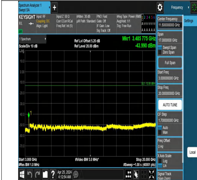
Band66_5MHz_QPSK_132322_1RB#0_3000~20000_3000~2000
