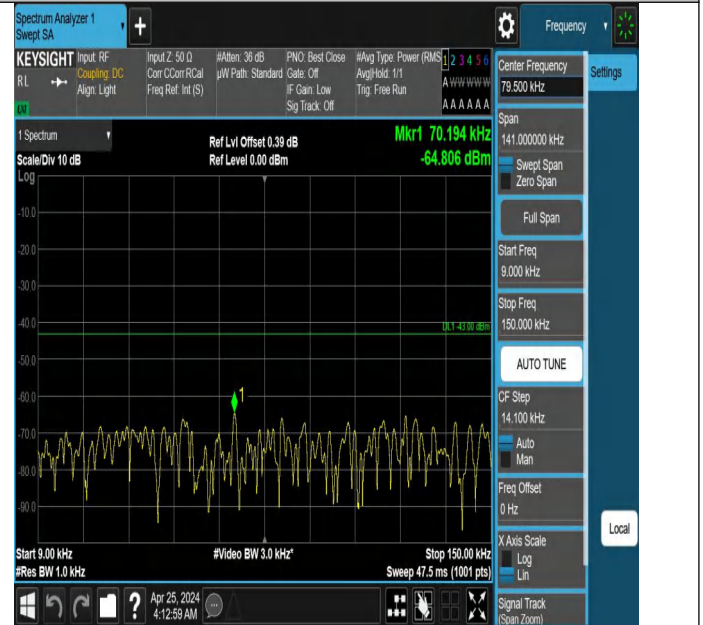
Band66_5MHz_QPSK_132322_1RB#24_0.009~0.15_0.009~0.15
