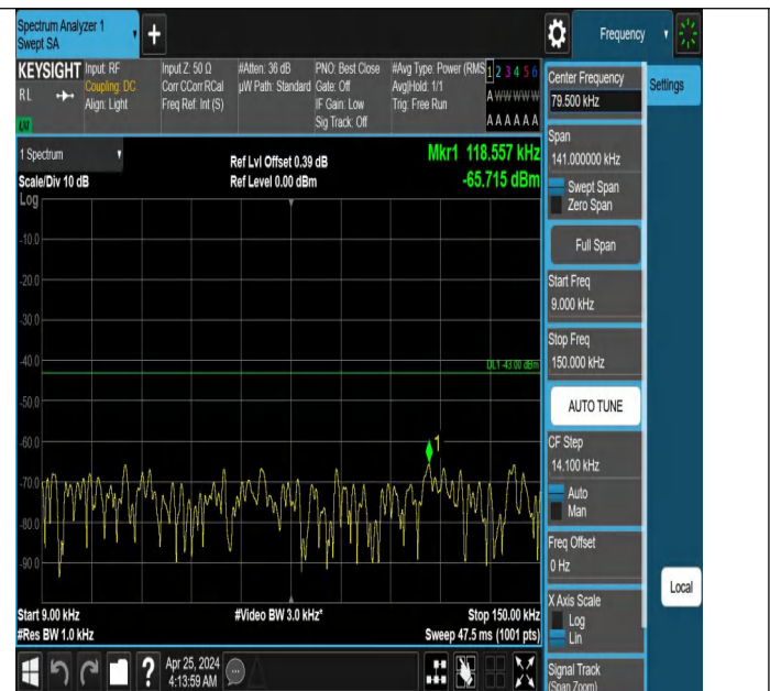
Band66_5MHz_QPSK_132647_1RB#24_0.009~0.15_0.009~0.15
