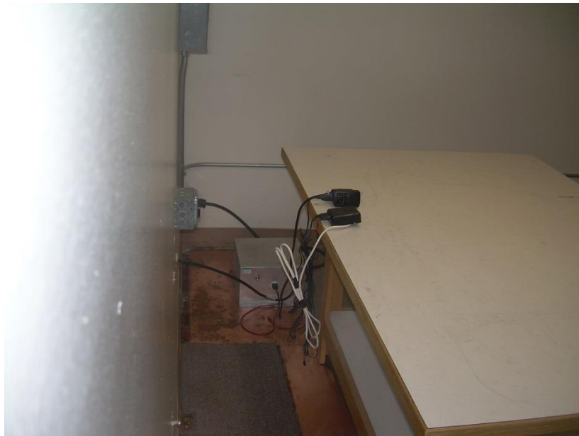
Photograph 10 - Back View Conducted Emissions Worst Case Configuration – C4-Z2IO
