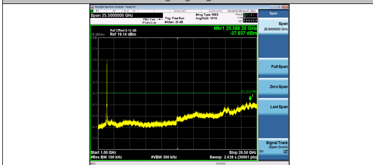
11N40SISO_Ant1_2437_0~Reference
